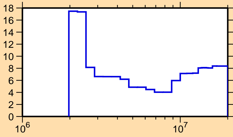
\Delta\sigma/\sigma vs. E for ^{198}\text{Hg}(n,n\text{cont.})
