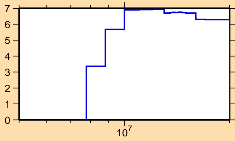
\Delta\sigma/\sigma vs. E for ^{198}\text{Hg}(n,\text{inel.})
