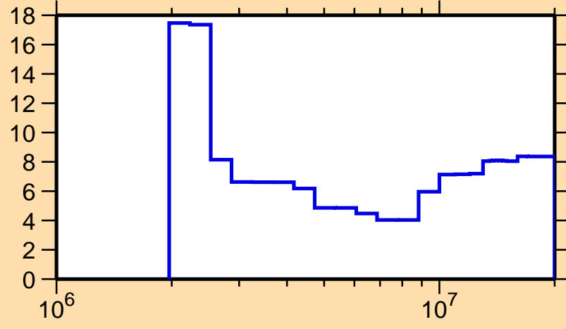
\Delta\sigma/\sigma vs. E for ^{198}\text{Hg}(n,n\text{cont.})
