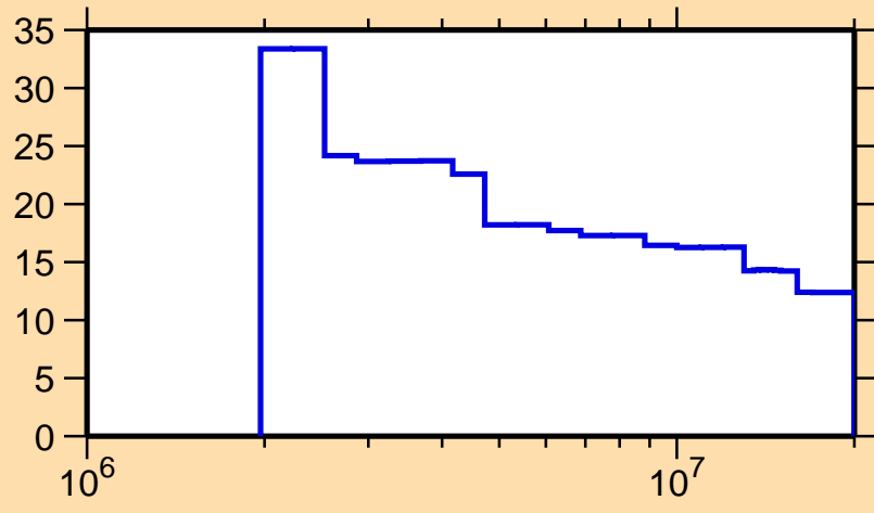
\Delta\sigma/\sigma vs. E for ^{198}\text{Hg}(n,n_1)
