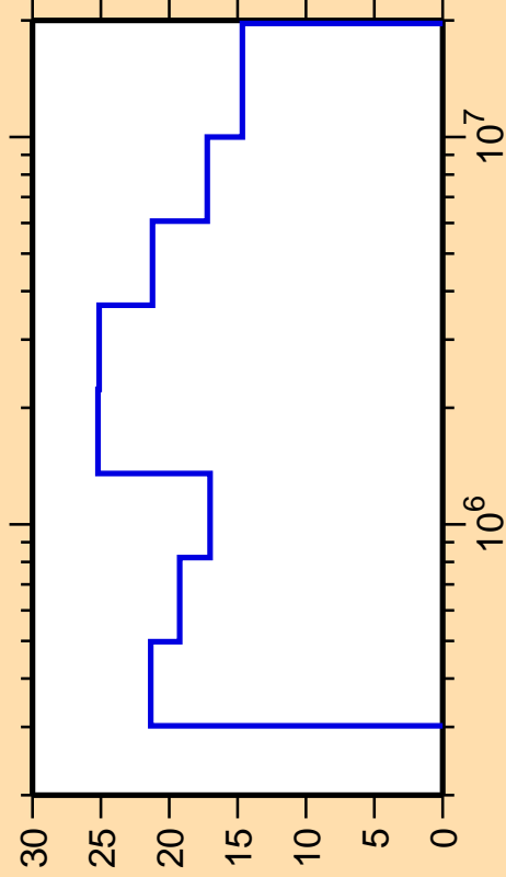
\Delta\sigma/\sigma vs. E for ^{198}\text{Hg}(n,n_1)
