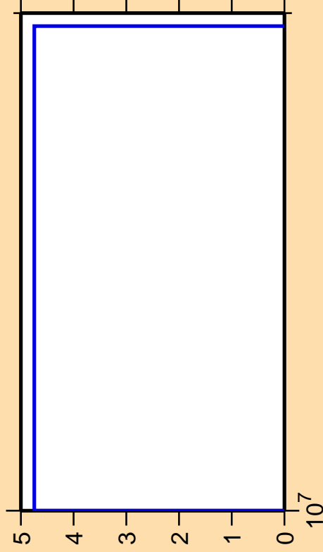
\Delta\sigma/\sigma vs. E for ^{198}\text{Hg}(n,2n\alpha)
