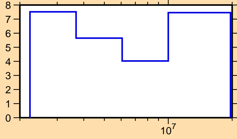
\Delta\sigma/\sigma vs. E for ^{198}\text{Hg}(n,n\text{cont.})
