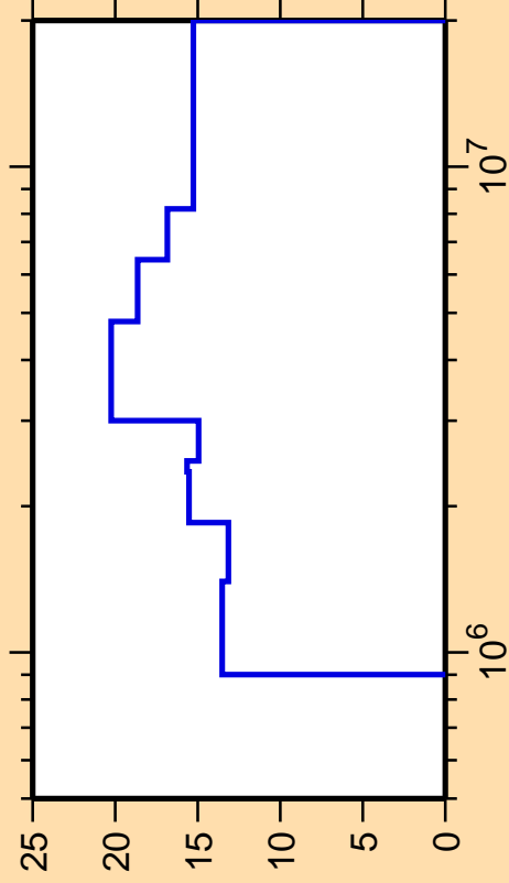
\Delta\sigma/\sigma vs. E for ^{198}\text{Hg}(n,n_3)
