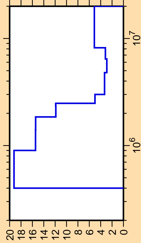
\Delta\sigma/\sigma vs. E for ^{198}\text{Hg}(n,\text{inel.})
