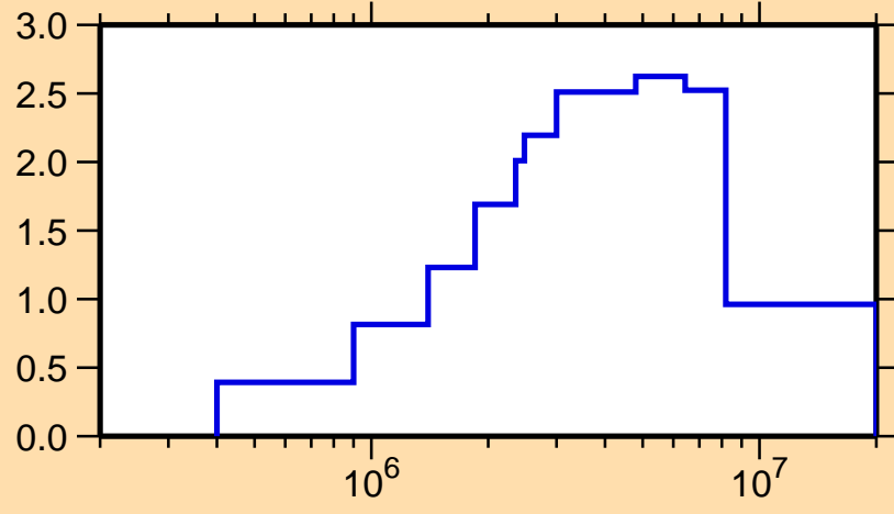
\sigma vs. E for ^{198}\text{Hg}(n,\text{inel.})
