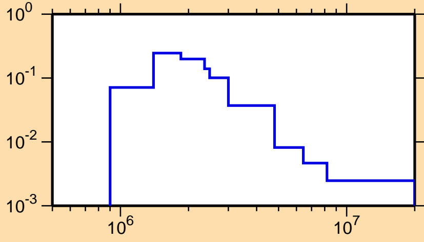
\sigma vs. E for ^{198}\text{Hg}(n,n_3)
