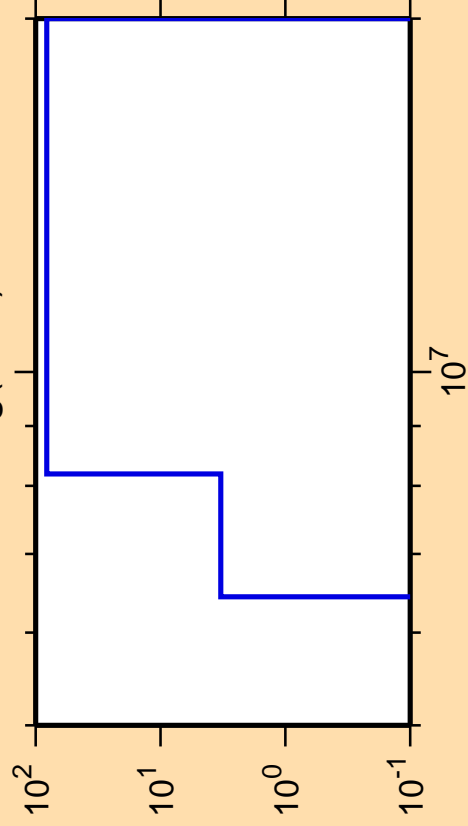
\Delta\sigma/\sigma vs. E for ^{198}\text{Hg}(n,n\alpha)
