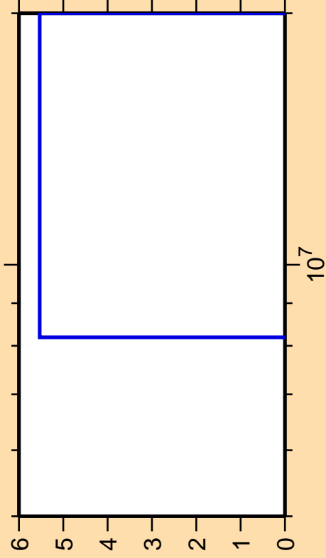
\Delta\sigma/\sigma vs. E for ^{198}\text{Hg}(n,\text{He}3)
