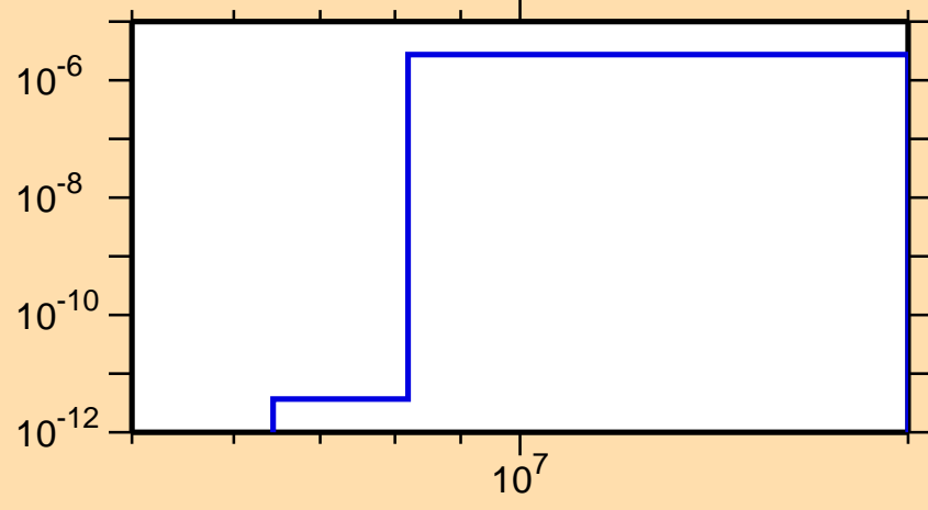
\sigma vs. E for ^{198}\text{Hg}(n,n\alpha)
