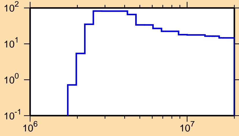
\Delta\sigma/\sigma vs. E for ^{199}\text{Hg}(n,p)
