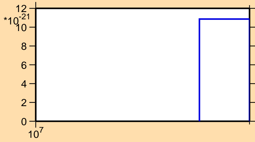
\sigma vs. E for ^{199}\text{Hg} (mt 11)
