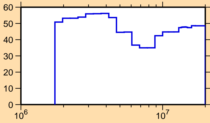
\Delta\sigma/\sigma vs. E for ^{199}\text{Hg}(n,\gamma)
