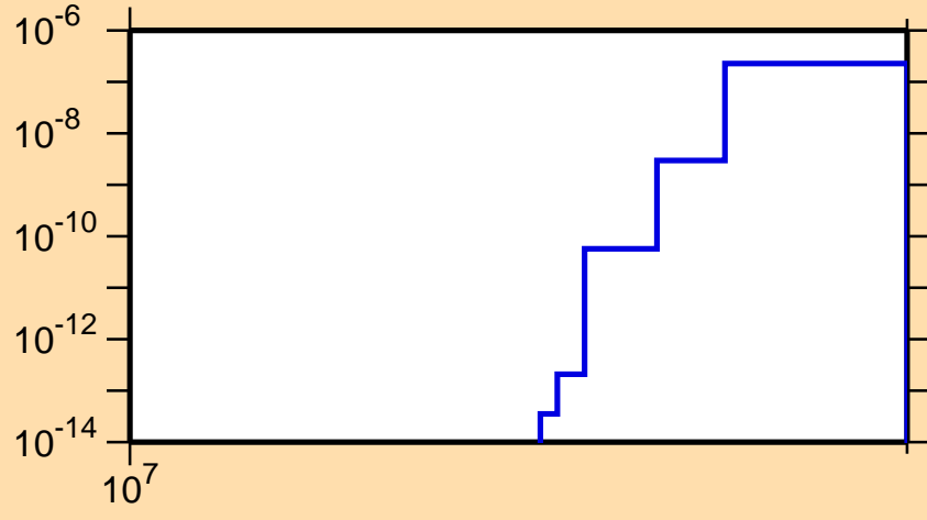
\sigma vs. E for ^{199}\text{Hg}(n,\text{nd})
