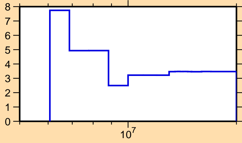
\Delta\sigma/\sigma vs. E for ^{199}\text{Hg}(n,\text{el.})
