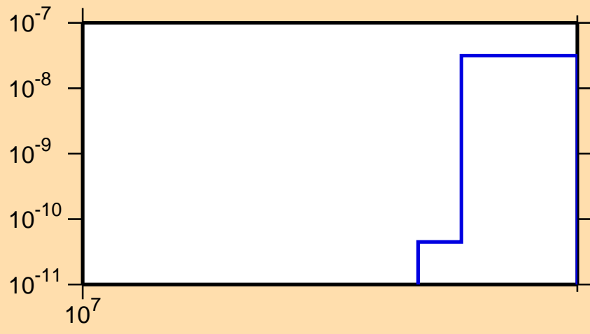
\sigma vs. E for ^{199}\text{Hg}(n,2np)
