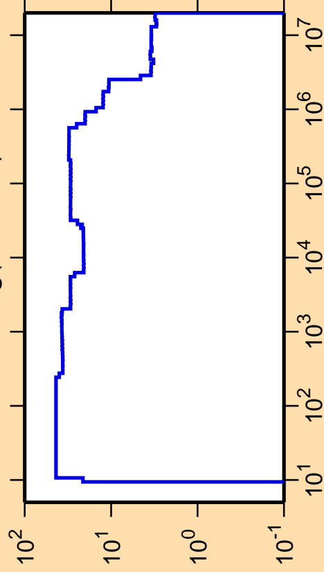
\Delta\sigma/\sigma vs. E for ^{199}\text{Hg}(n,\text{nonel.})
