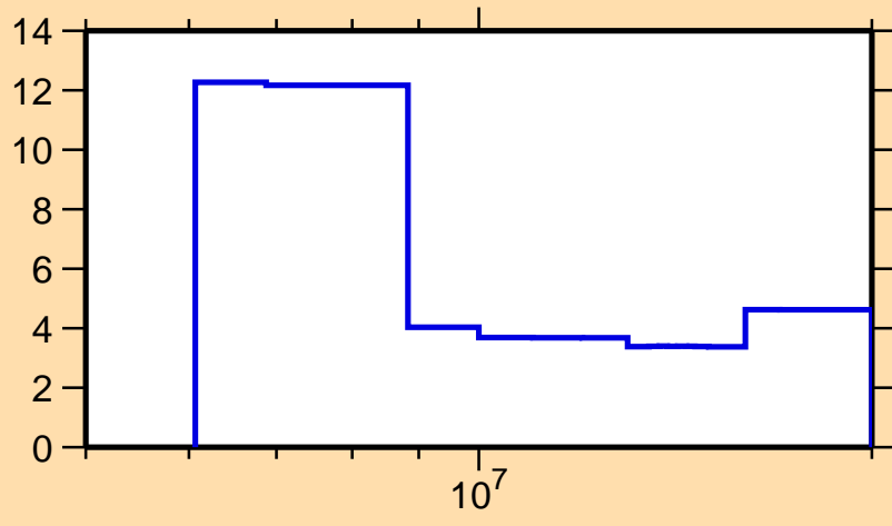
\Delta\sigma/\sigma vs. E for ^{199}\text{Hg}(n,2n)
