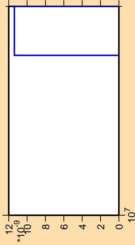
\Delta\sigma/\sigma vs. E for ^{199}\text{Hg} (mt 11)
