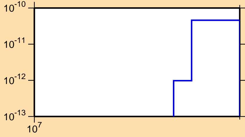
\sigma vs. E for ^{199}\text{Hg}(n,\text{He}3)
