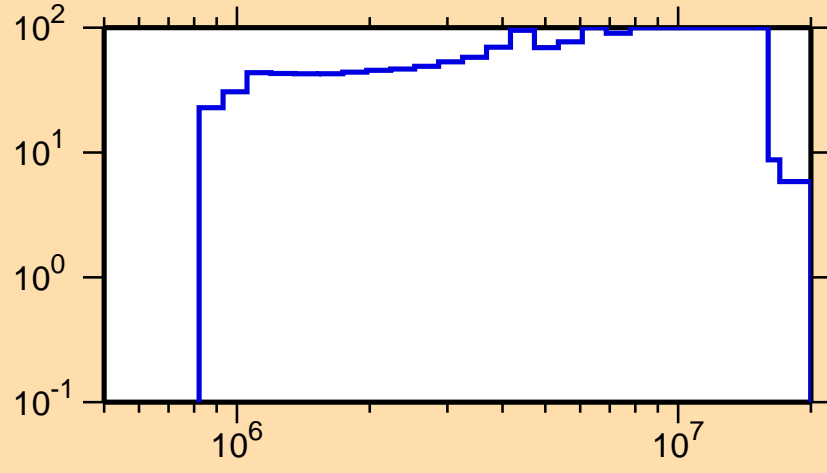
\Delta\sigma/\sigma vs. E for ^{199}\text{Hg}(n,n_1)
