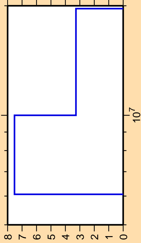
\Delta\sigma/\sigma vs. E for ^{199}\text{Hg}(n,2n)
