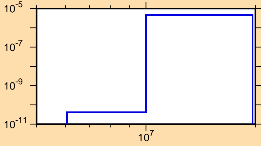
\sigma vs. E for ^{199}\text{Hg}(n,n\alpha)
