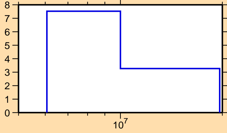
\Delta\sigma/\sigma vs. E for ^{199}\text{Hg}(n,2n)
