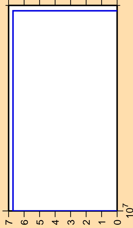
\Delta\sigma/\sigma vs. E for ^{199}\text{Hg}(n,3n)
