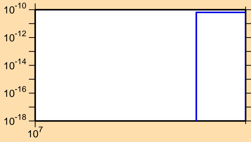
\sigma vs. E for ^{200}\text{Hg}(n,2np)
