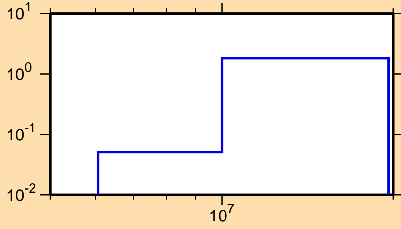
\sigma vs. E for ^{200}\text{Hg}(n,2n)
