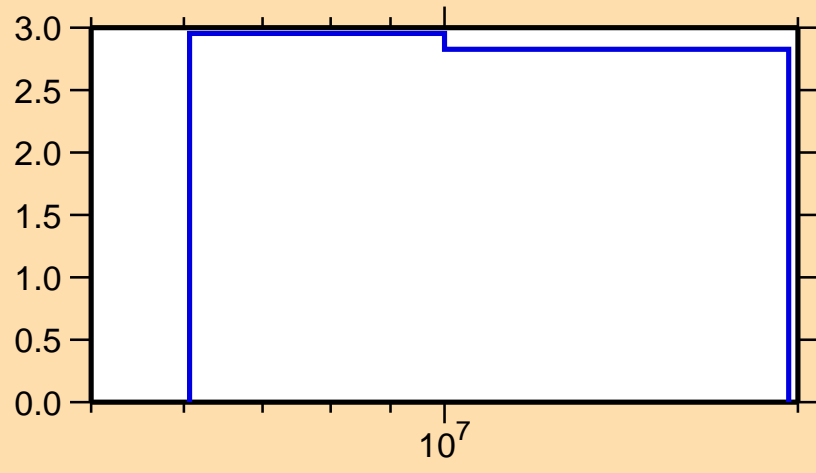
\Delta\sigma/\sigma vs. E for ^{200}\text{Hg}(n,\text{nonel.})
