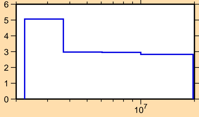
\Delta\sigma/\sigma vs. E for ^{200}\text{Hg}(n,\text{nonel.})
