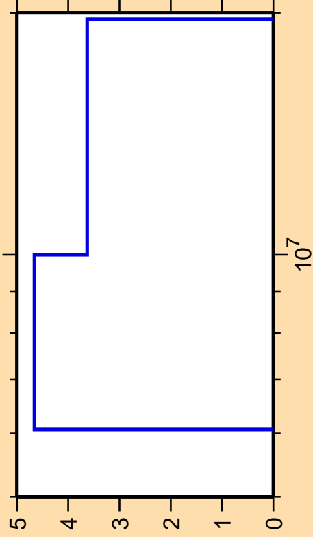
\Delta\sigma/\sigma vs. E for ^{200}\text{Hg}(n,2n)
