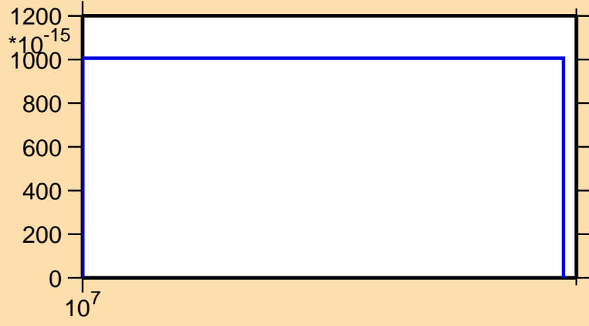
\sigma vs. E for ^{200}\text{Hg}(n,nt)
