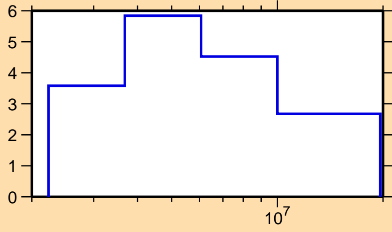
\Delta\sigma/\sigma vs. E for ^{200}\text{Hg}(n,\text{el.})
