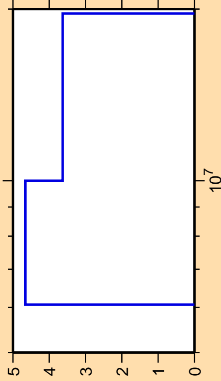
\Delta\sigma/\sigma vs. E for ^{200}\text{Hg}(n,2n)
