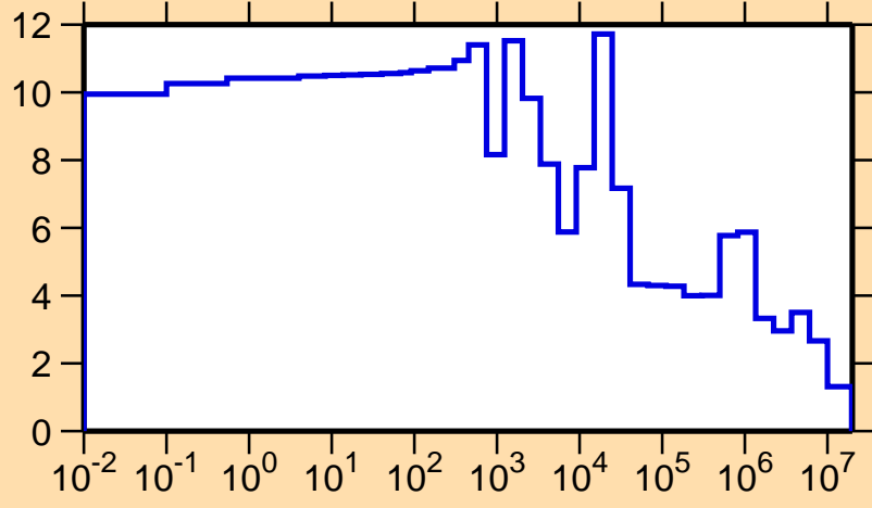
\Delta\sigma/\sigma vs. E for ^{200}\text{Hg}(n,\text{tot.})
