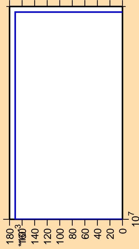
\Delta\sigma/\sigma vs. E for ^{200}\text{Hg}(n,\text{He}3)
