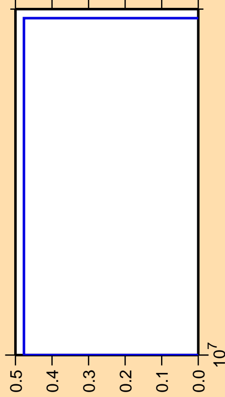
\Delta\sigma/\sigma vs. E for ^{200}\text{Hg}(n,2np)
