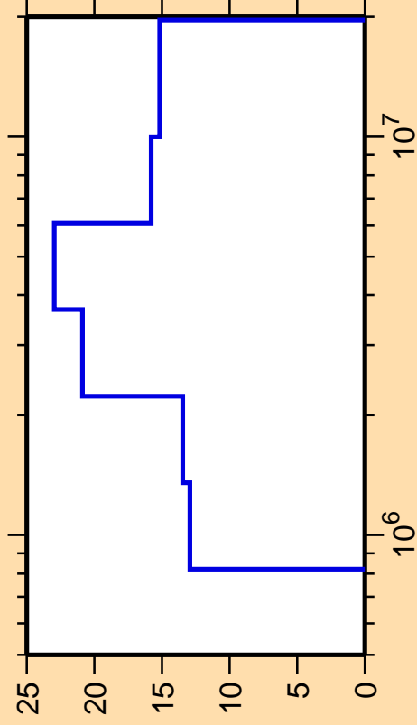
\Delta\sigma/\sigma vs. E for ^{200}\text{Hg}(n,n_4)
