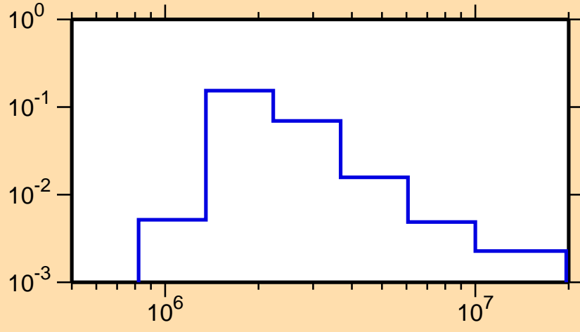
\sigma vs. E for ^{200}\text{Hg}(n,n_4)
