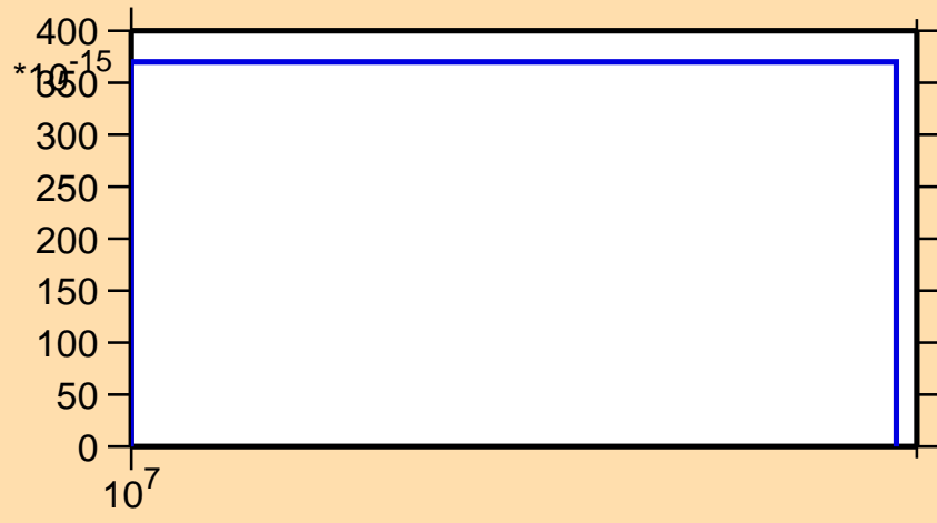
\sigma vs. E for ^{200}\text{Hg}(n,2np)
