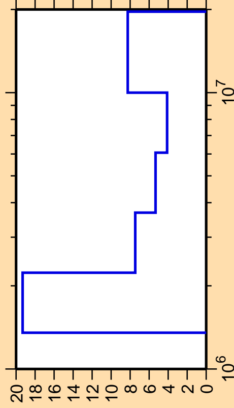
\Delta\sigma/\sigma vs. E for ^{200}\text{Hg}(n,n\text{cont.})
