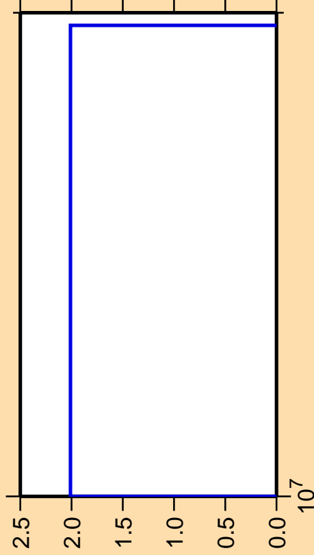
\Delta\sigma/\sigma vs. E for ^{200}\text{Hg}(n,nt)
