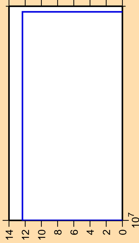
\Delta\sigma/\sigma vs. E for ^{200}\text{Hg}(n,3n)
