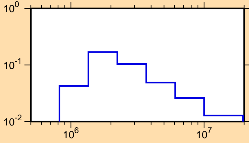
\sigma vs. E for ^{200}\text{Hg}(n,n_2)
