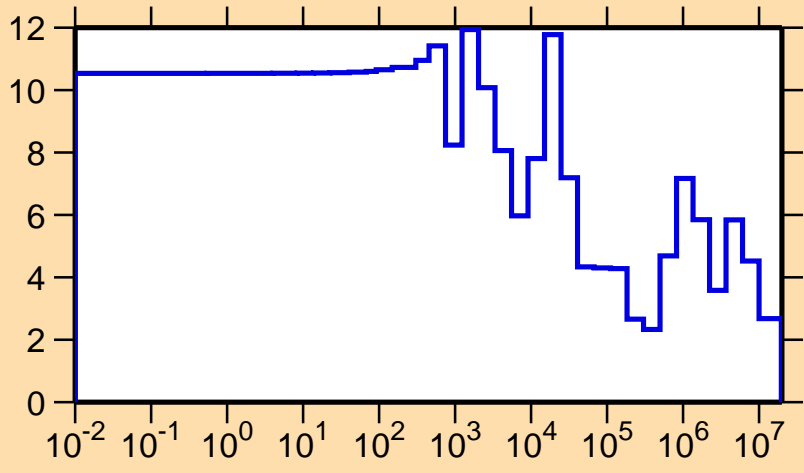
\Delta\sigma/\sigma vs. E for ^{200}\text{Hg}(n,\text{el.})
