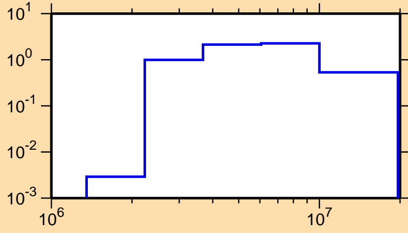
\sigma vs. E for ^{200}\text{Hg}(n,n\text{cont.})
