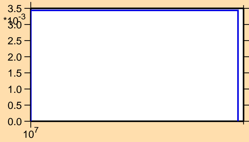
\sigma vs. E for ^{200}\text{Hg}(n,3n)
