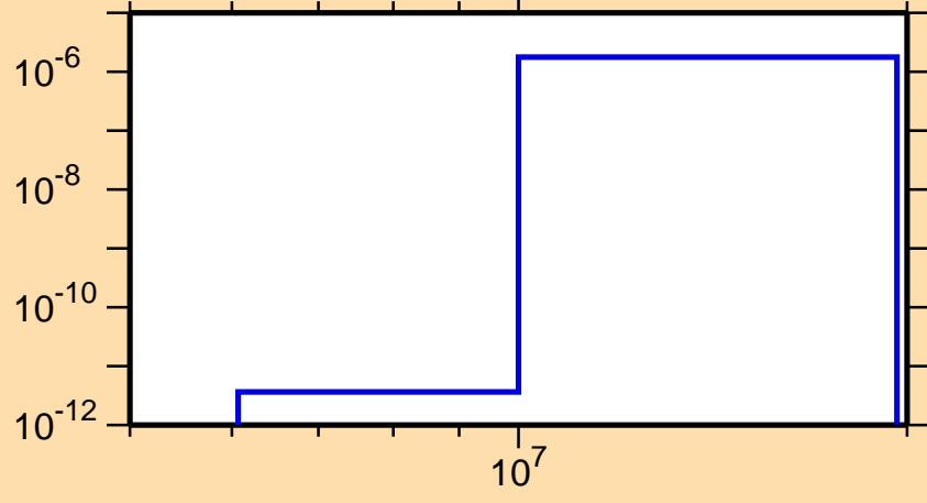
\sigma vs. E for ^{200}\text{Hg}(n,n\alpha)
