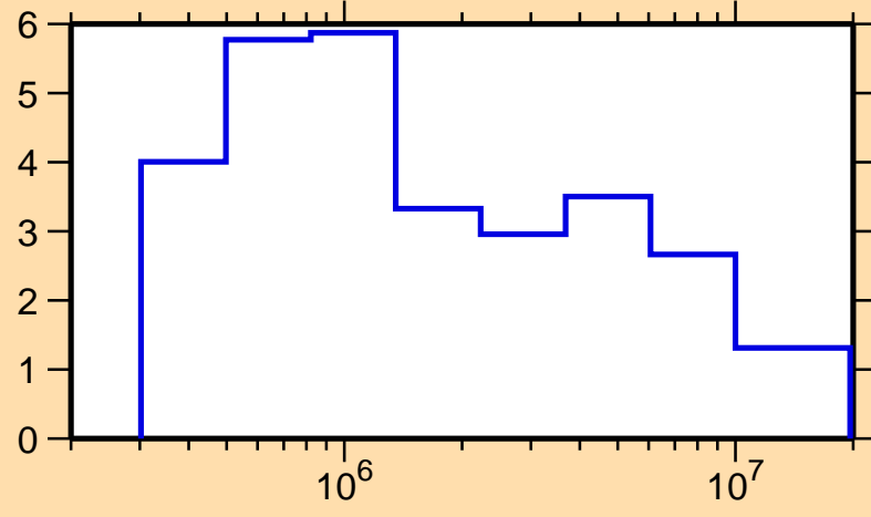
\Delta\sigma/\sigma vs. E for ^{200}\text{Hg}(n,\text{tot.})
