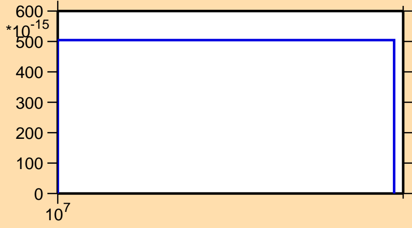
\sigma vs. E for ^{200}\text{Hg}(n,2n\alpha)
