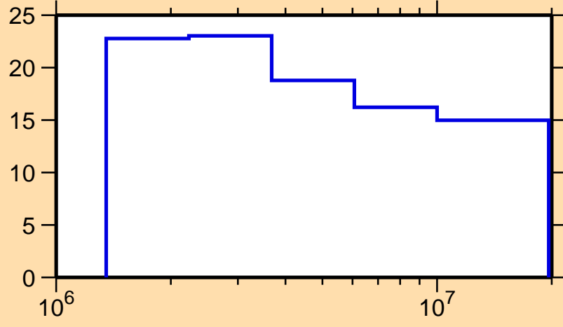
\Delta\sigma/\sigma vs. E for ^{200}\text{Hg}(n,n_1)
