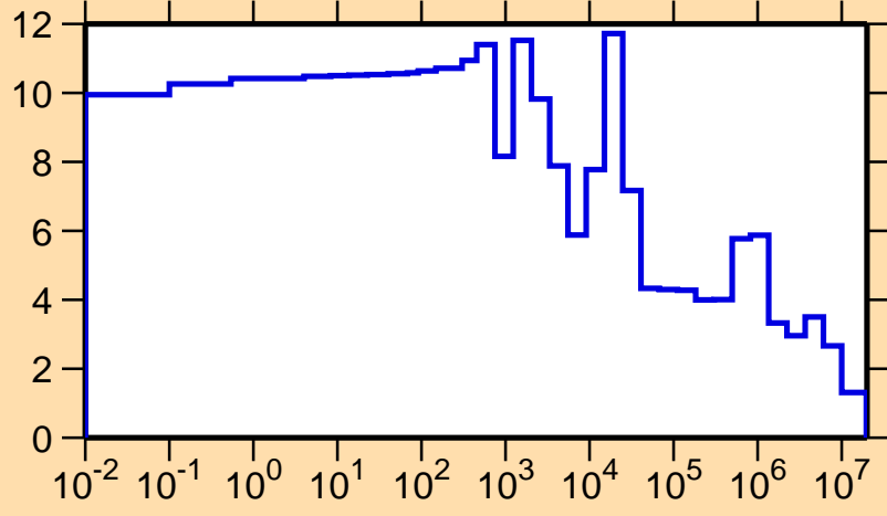
\Delta\sigma/\sigma vs. E for ^{200}\text{Hg}(n,\text{tot.})
