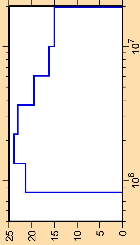
\Delta\sigma/\sigma vs. E for ^{200}\text{Hg}(n,n_2)
