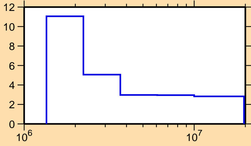
\Delta\sigma/\sigma vs. E for ^{200}\text{Hg}(n,\text{nonel.})
