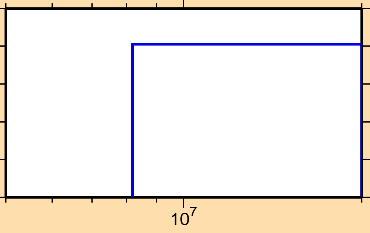
\sigma vs. E for ^{200}\text{Hg}(n,\text{nd})
