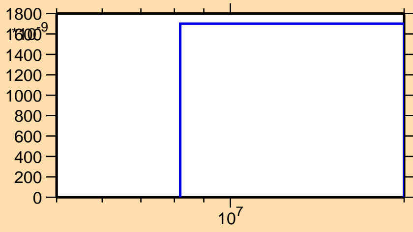
\sigma vs. E for ^{200}\text{Hg}(n,t)
