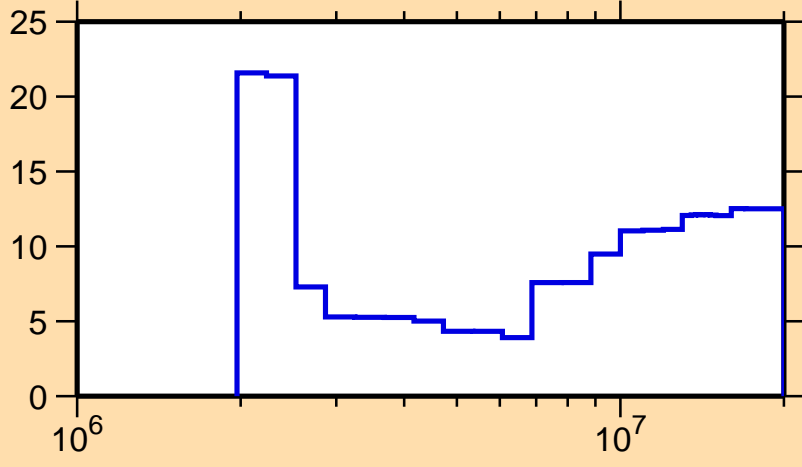
\Delta\sigma/\sigma vs. E for ^{201}\text{Hg}(n,n\text{cont.})
