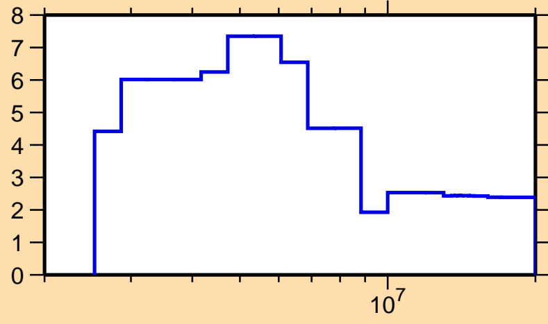
\Delta\sigma/\sigma vs. E for ^{201}\text{Hg}(n,\text{el.})
