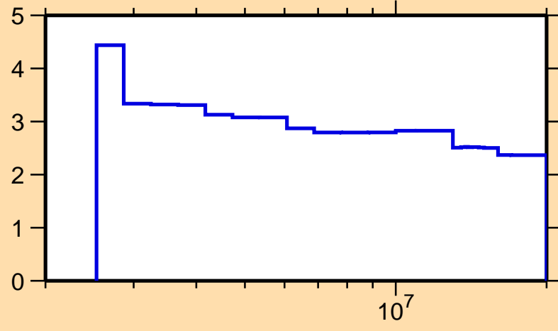
\Delta\sigma/\sigma vs. E for ^{201}\text{Hg}(n,\text{nonel.})
