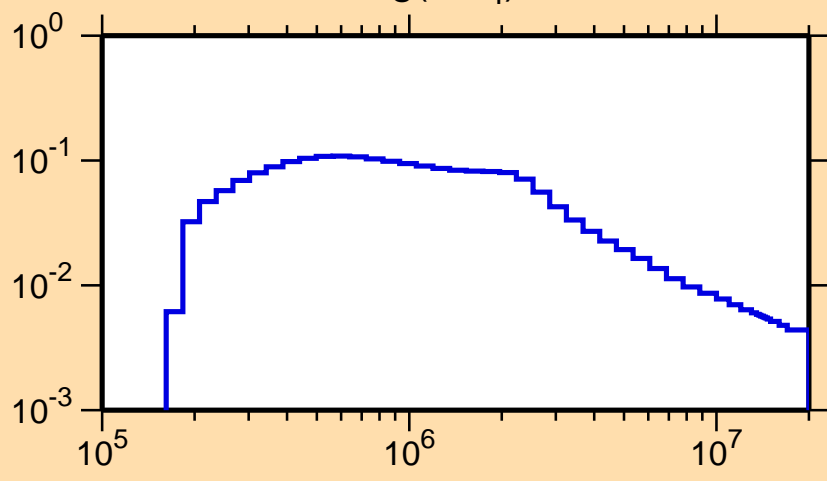
\sigma vs. E for ^{201}\text{Hg}(n,n_4)
