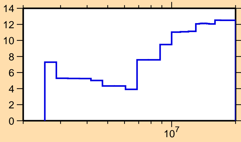
\Delta\sigma/\sigma vs. E for ^{201}\text{Hg}(n,n\text{cont.})
