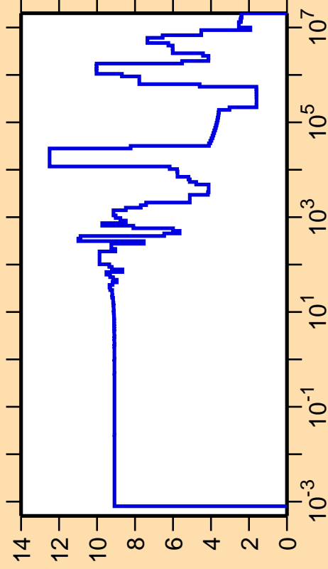
\Delta\sigma/\sigma vs. E for ^{201}\text{Hg}(n,\text{el.})
