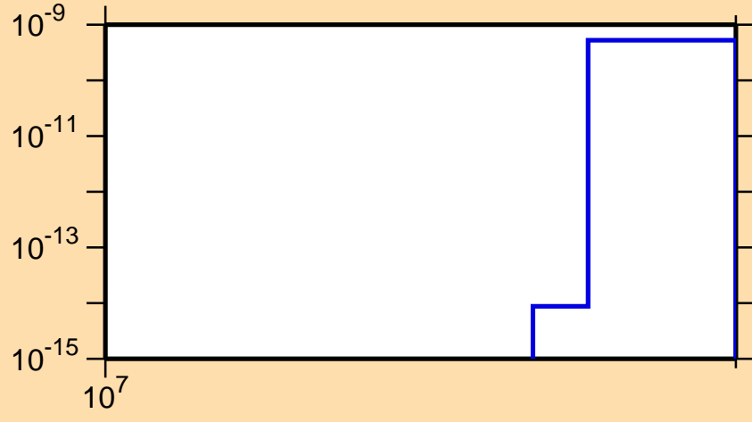
\sigma vs. E for ^{201}\text{Hg}(n,nt)
