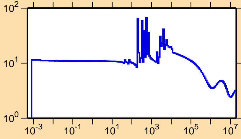
\sigma vs. E for ^{201}\text{Hg}(n,\text{el.})
