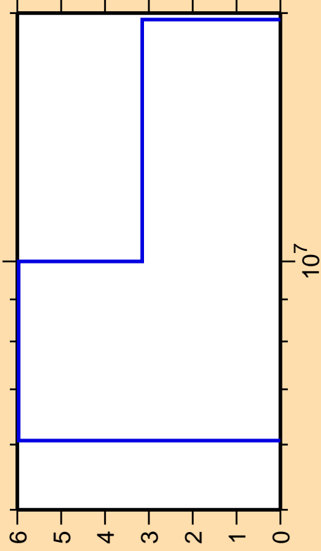
\Delta\sigma/\sigma vs. E for ^{201}\text{Hg}(n,2n)
