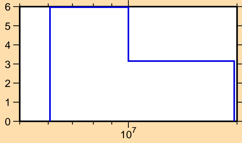
\Delta\sigma/\sigma vs. E for ^{201}\text{Hg}(n,2n)
