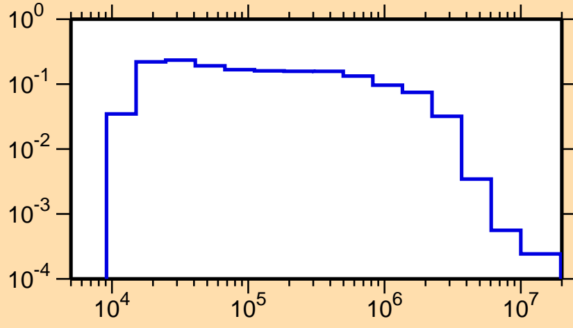
\sigma vs. E for ^{201}\text{Hg}(n,n_1)
