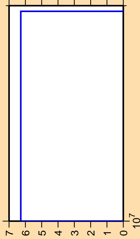
\Delta\sigma/\sigma vs. E for ^{201}\text{Hg}(n,nt)
