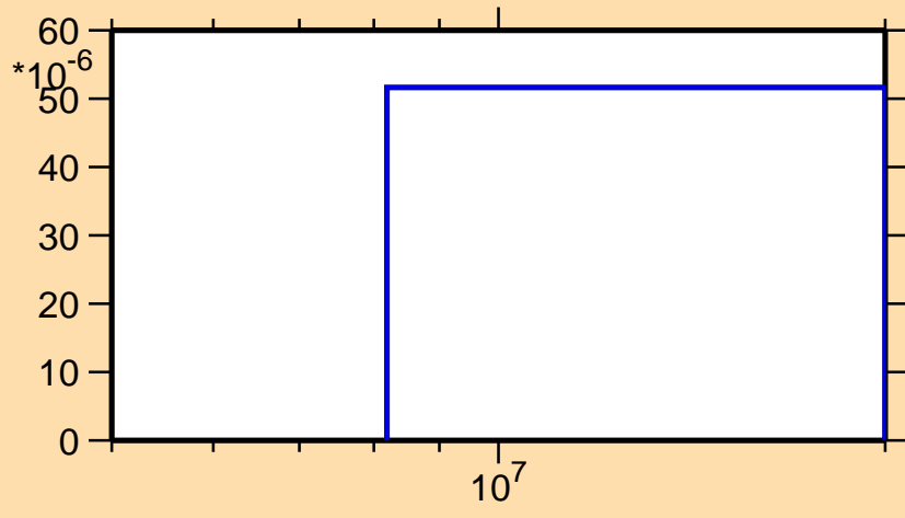
\sigma vs. E for ^{201}\text{Hg}(n,d)
