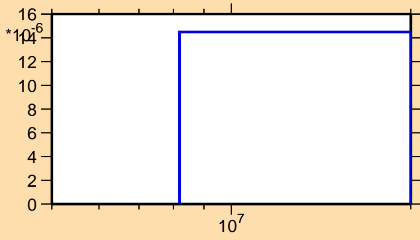
\sigma vs. E for ^{201}\text{Hg}(n,t)
