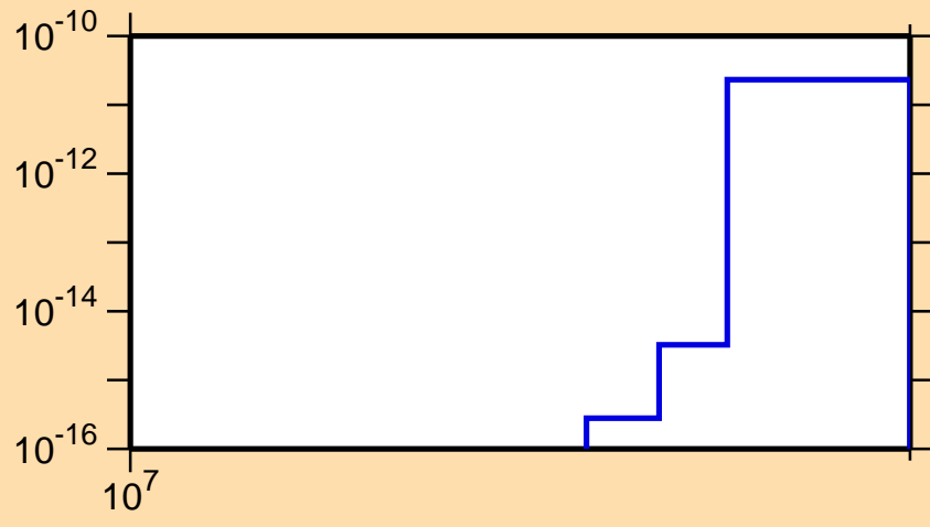
\sigma vs. E for ^{202}\text{Hg}(n,2np)
