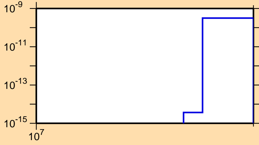
\sigma vs. E for ^{202}\text{Hg}(n,nt)
