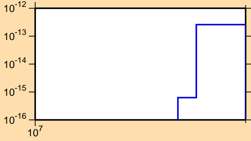
\sigma vs. E for ^{202}\text{Hg}(n,\text{He}3)
