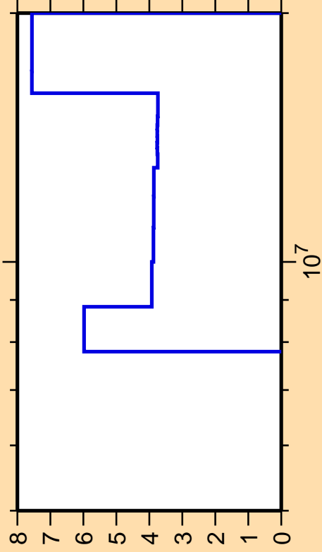
\Delta\sigma/\sigma vs. E for ^{202}\text{Hg}(n,2n)
