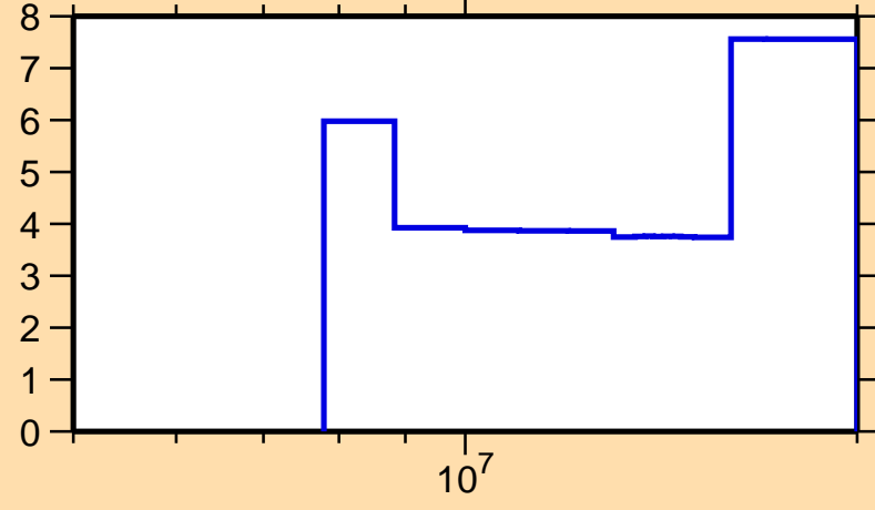
\Delta\sigma/\sigma vs. E for ^{202}\text{Hg}(n,2n)
