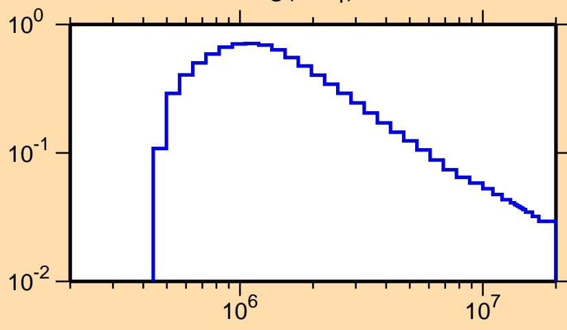
\sigma vs. E for ^{202}\text{Hg}(n,n_1)
