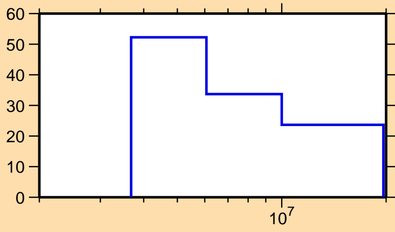
\Delta\sigma/\sigma vs. E for ^{202}\text{Hg}(n,p)
