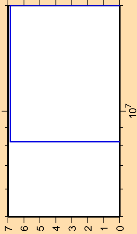
\Delta\sigma/\sigma vs. E for ^{202}\text{Hg}(n,nt)
