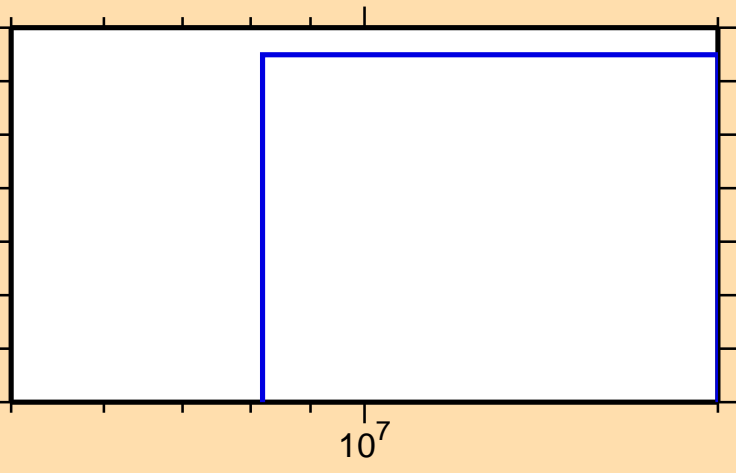
\sigma vs. E for ^{202}\text{Hg}(n,\text{nd})
