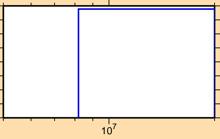
\sigma vs. E for ^{202}\text{Hg}(n,d)
