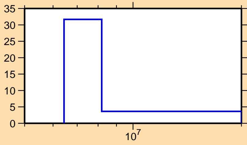
\Delta\sigma/\sigma vs. E for ^{202}\text{Hg}(n,2n)
