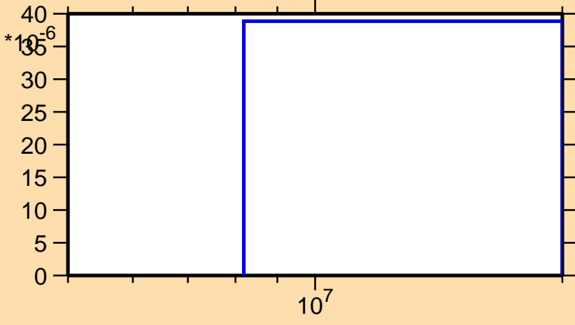
\sigma vs. E for ^{202}\text{Hg}(n,d)
