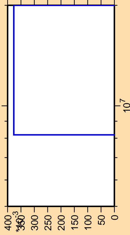
\Delta\sigma/\sigma vs. E for ^{202}\text{Hg}(n,2np)
