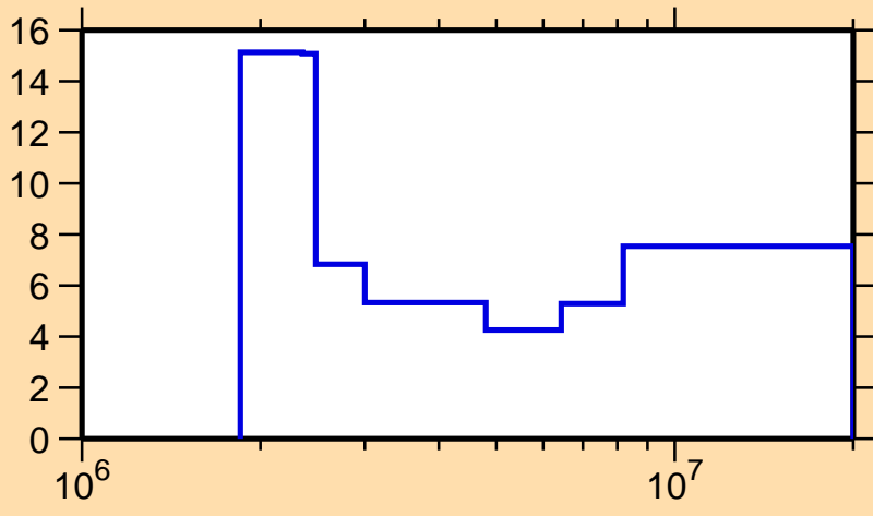
\Delta\sigma/\sigma vs. E for ^{202}\text{Hg}(n,n\text{cont.})
