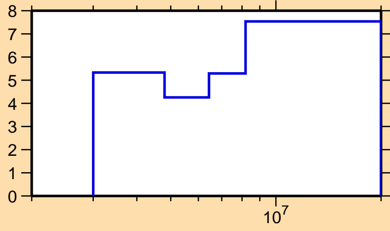
\Delta\sigma/\sigma vs. E for ^{202}\text{Hg}(n,n\text{cont.})
