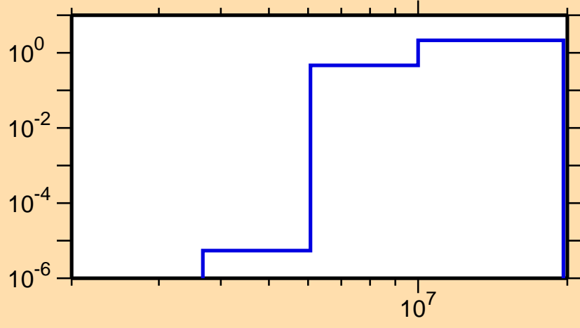
\sigma vs. E for ^{203}\text{Hg}(n,2n)
