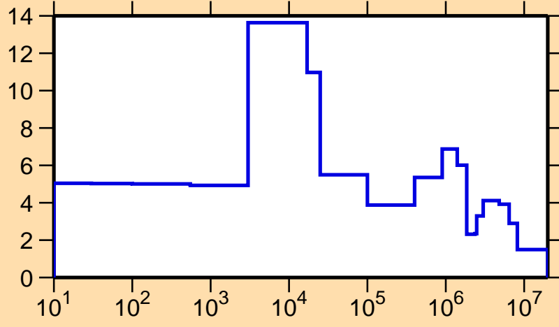
\Delta\sigma/\sigma vs. E for ^{203}\text{Hg}(n,\text{tot.})
