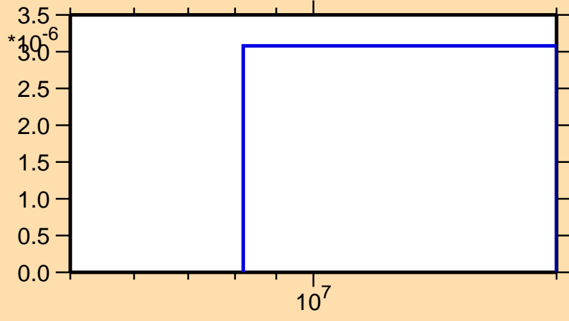
\sigma vs. E for ^{203}\text{Hg}(n,t)
