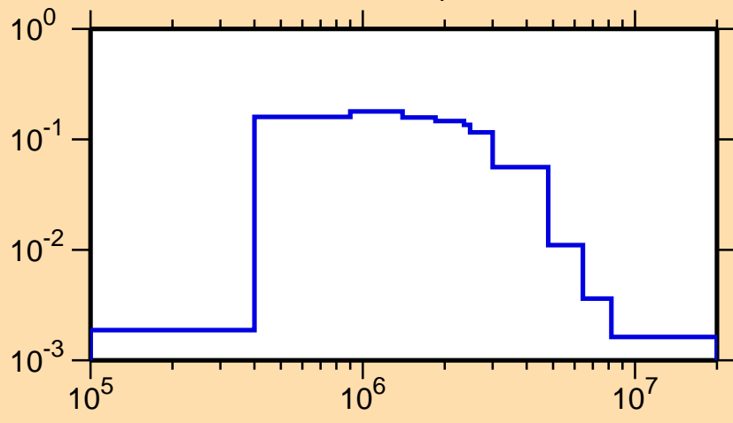
\sigma vs. E for ^{203}\text{Hg}(n,n_4)
