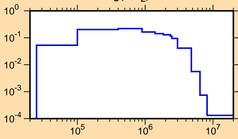
\sigma vs. E for ^{203}\text{Hg}(n,n_2)
