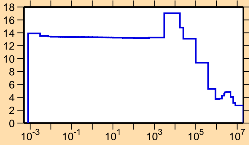
\sigma vs. E for ^{203}\text{Hg}(n,\text{el.})
