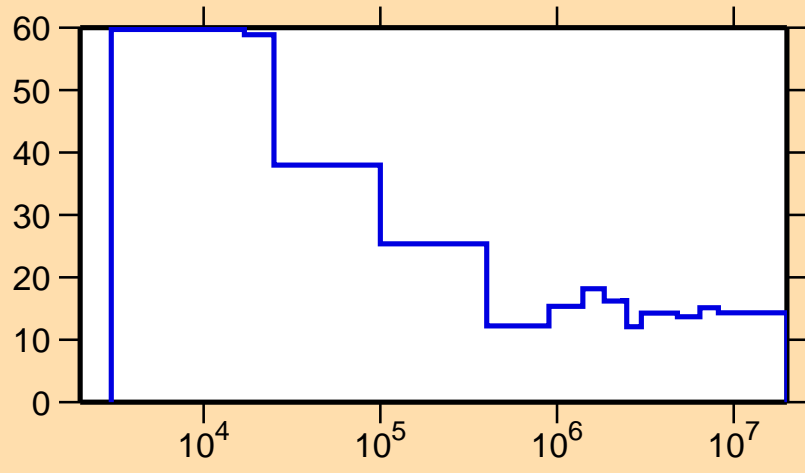
\Delta\sigma/\sigma vs. E for ^{203}\text{Hg}(n,n_1)
