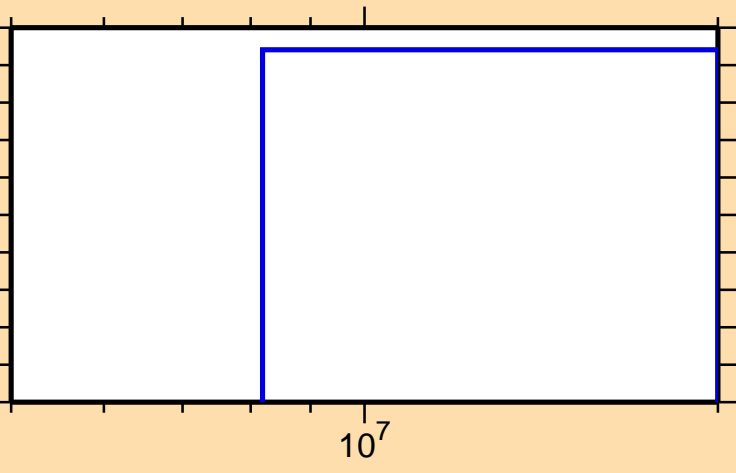
\sigma vs. E for ^{203}\text{Hg}(n,np)
