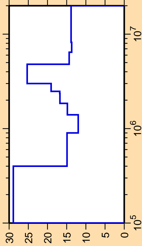
\Delta\sigma/\sigma vs. E for ^{203}\text{Hg}(n,n_4)
