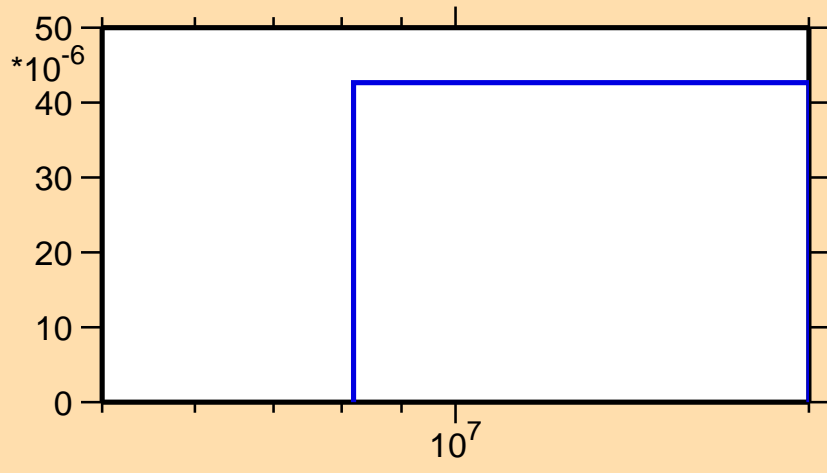
\sigma vs. E for ^{203}\text{Hg}(n,d)
