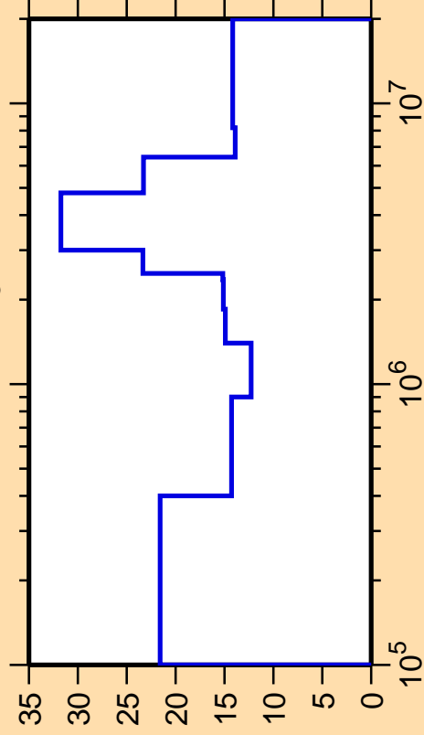
\Delta\sigma/\sigma vs. E for ^{203}\text{Hg}(n,n_3)
