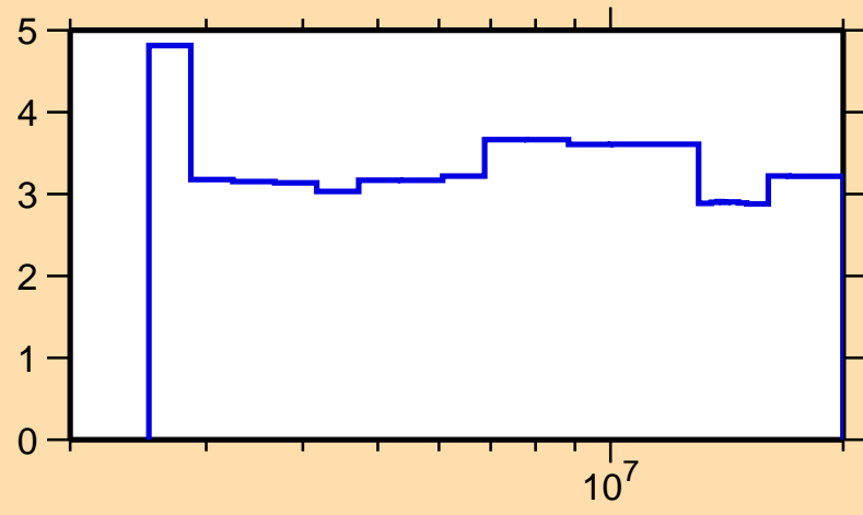
\Delta\sigma/\sigma vs. E for ^{204}\text{Hg}(n,n\text{onel.})
