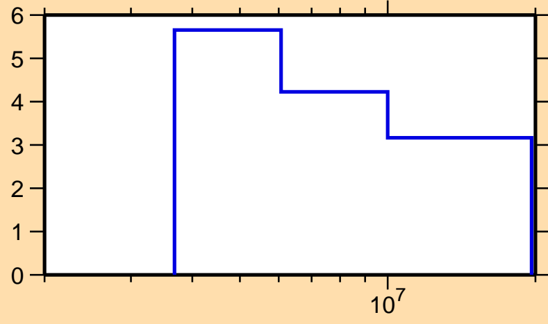
\Delta\sigma/\sigma vs. E for ^{204}\text{Hg}(n,\text{el.})
