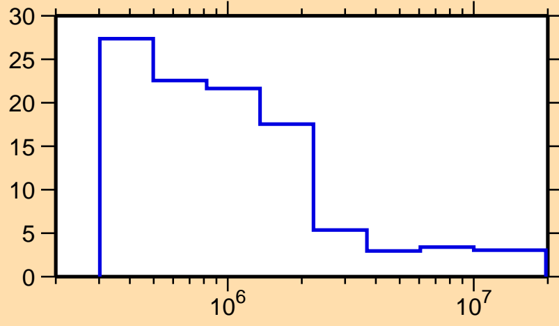
\Delta\sigma/\sigma vs. E for ^{204}\text{Hg}(n,\text{nonel.})
