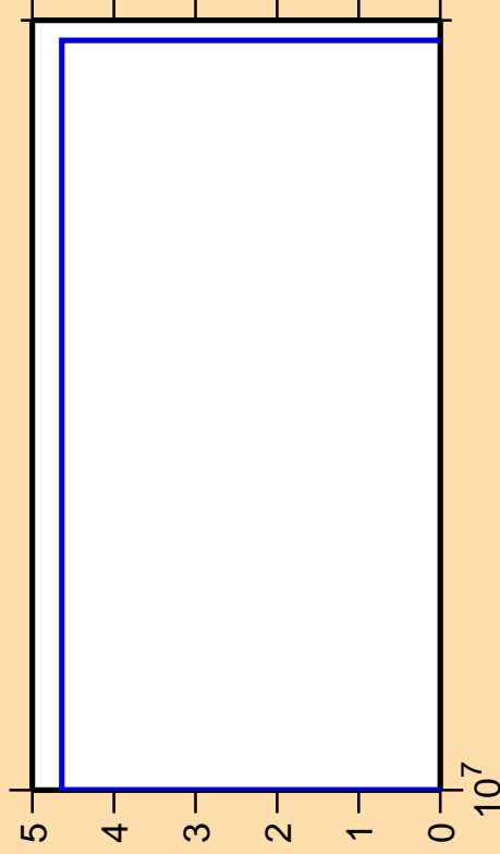
\Delta\sigma/\sigma vs. E for ^{204}\text{Hg}(n,nt)
