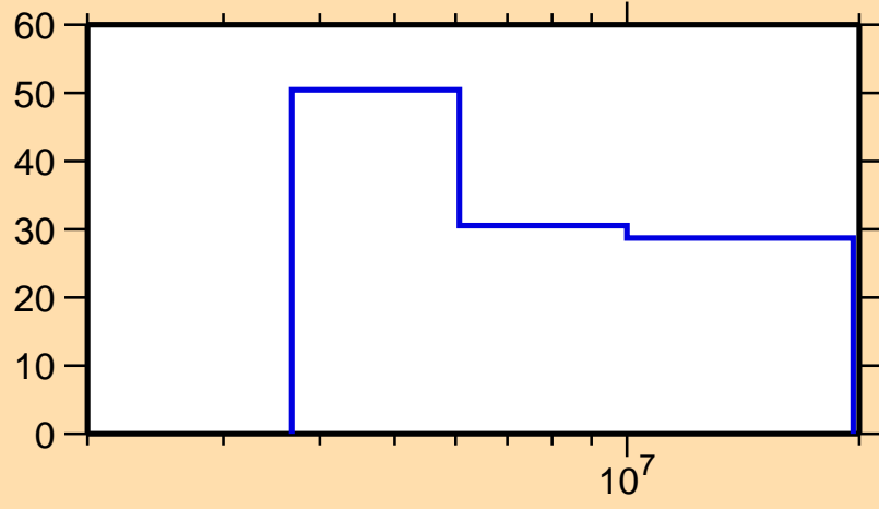
\Delta\sigma/\sigma vs. E for ^{204}\text{Hg}(n,\gamma)
