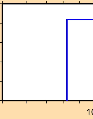
\sigma vs. E for ^{204}\text{Hg}(n,np)
