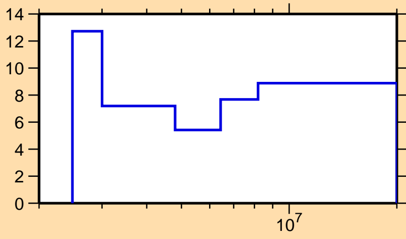
\Delta\sigma/\sigma vs. E for ^{204}\text{Hg}(n,n\text{cont.})
