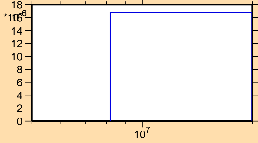
\sigma vs. E for ^{204}\text{Hg}(n,d)
