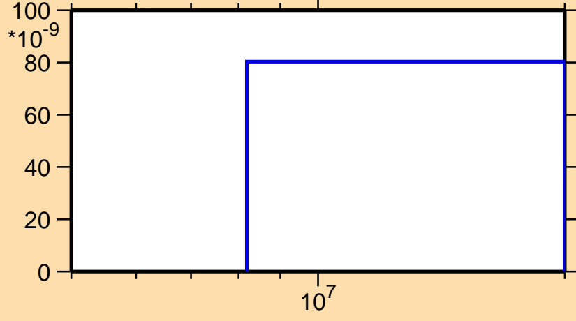
\sigma vs. E for ^{204}\text{Hg}(n,n\alpha)
