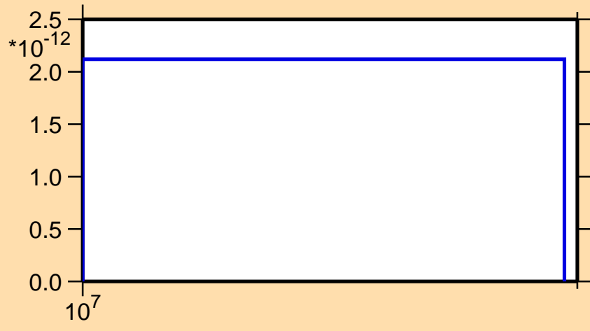
\sigma vs. E for ^{205}\text{Hg}(n,2np)
