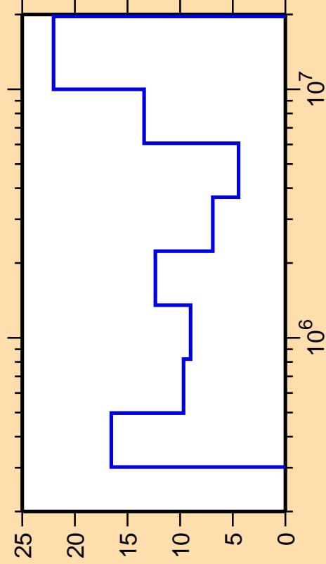
\Delta\sigma/\sigma vs. E for ^{205}\text{Hg}(n,\text{inel.})
