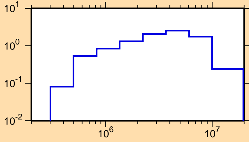
\sigma vs. E for ^{205}\text{Hg}(n,\text{inel.})
