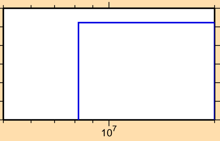
\sigma vs. E for ^{205}\text{Hg}(n,d)
