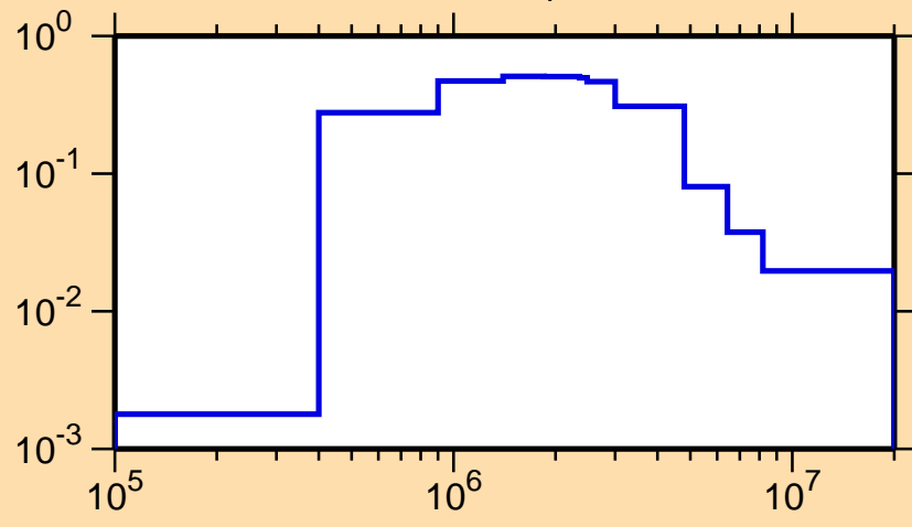
\sigma vs. E for ^{205}\text{Hg}(n,n_1)
