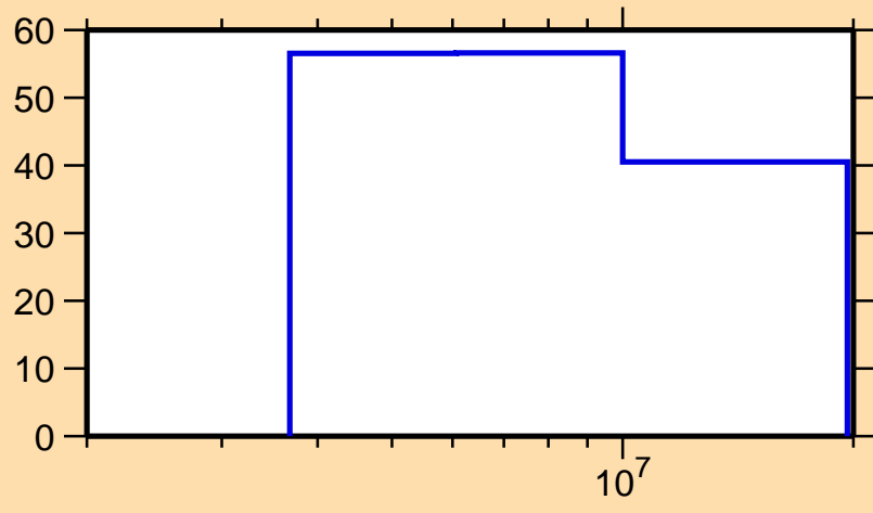
\Delta\sigma/\sigma vs. E for ^{206}\text{Hg}(n,\gamma)
