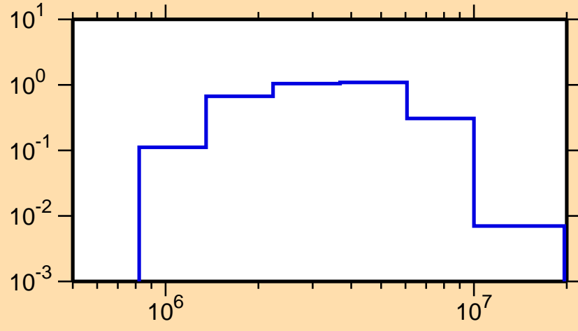
\sigma vs. E for ^{206}\text{Hg}(n,n_1)
