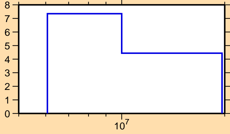
\Delta\sigma/\sigma vs. E for ^{206}\text{Hg}(n,2n)
