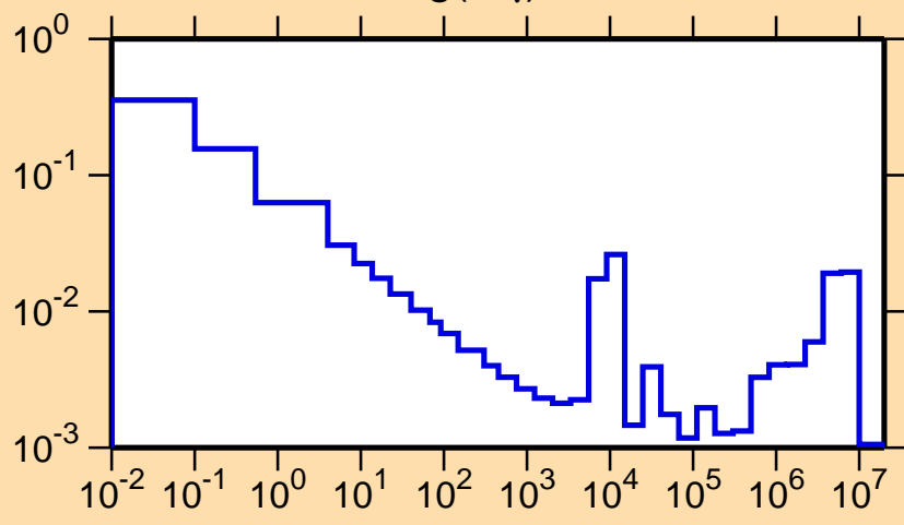
\sigma vs. E for ^{206}\text{Hg}(n,\gamma)
