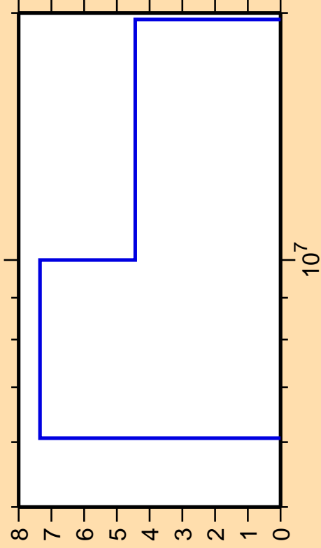
\Delta\sigma/\sigma vs. E for ^{206}\text{Hg}(n,2n)
