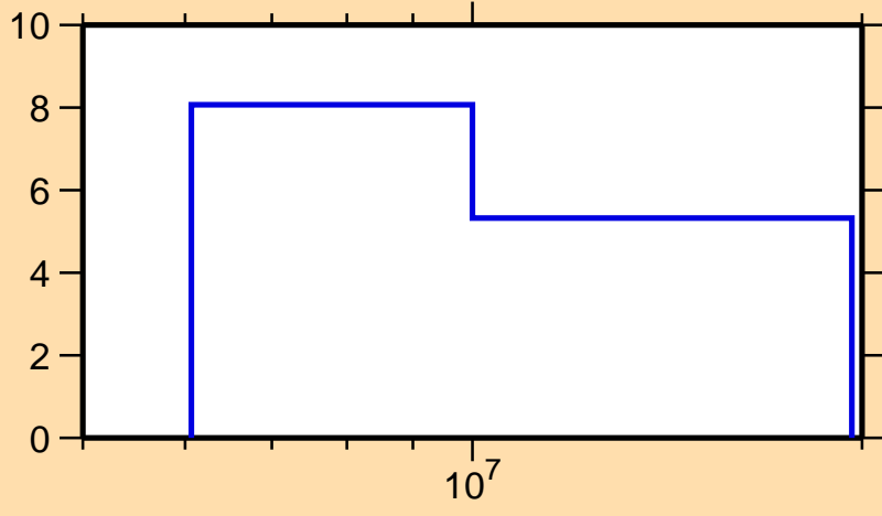
\Delta\sigma/\sigma vs. E for ^{207}\text{Hg}(n,\text{nonel.})
