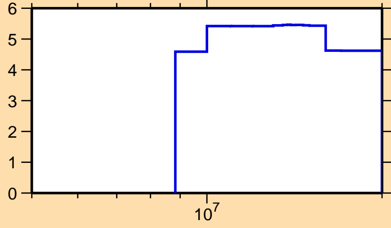
\Delta\sigma/\sigma vs. E for ^{208}\text{Hg}(n,\text{el.})
