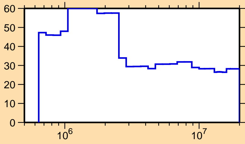
\Delta\sigma/\sigma vs. E for ^{208}\text{Hg}(n,n_1)
