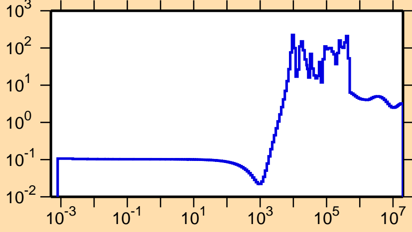
\sigma vs. E for ^{208}\text{Hg}(n,\text{el.})
