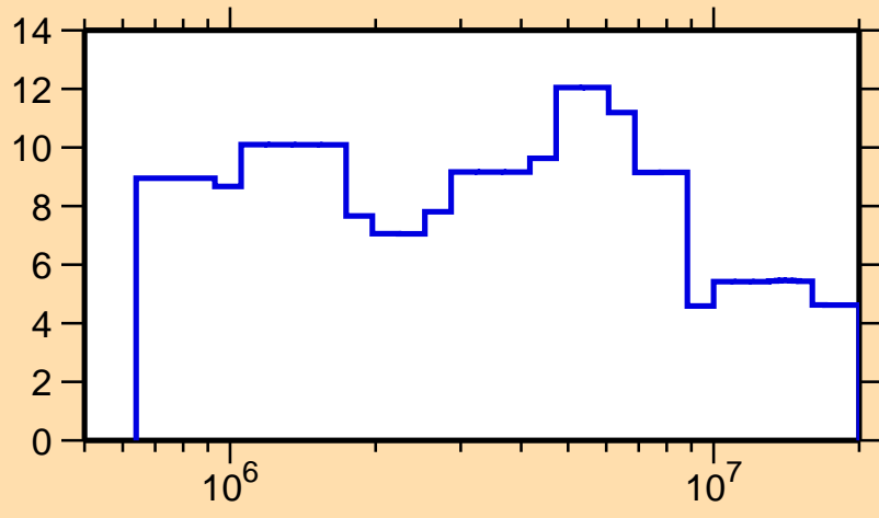
\Delta\sigma/\sigma vs. E for ^{208}\text{Hg}(n,\text{el.})
