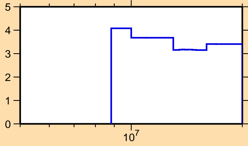
\Delta\sigma/\sigma vs. E for ^{208}\text{Hg}(n,\text{tot.})
