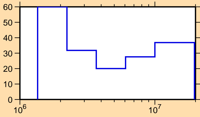
\Delta\sigma/\sigma vs. E for ^{208}\text{Hg}(n,n\text{cont.})
