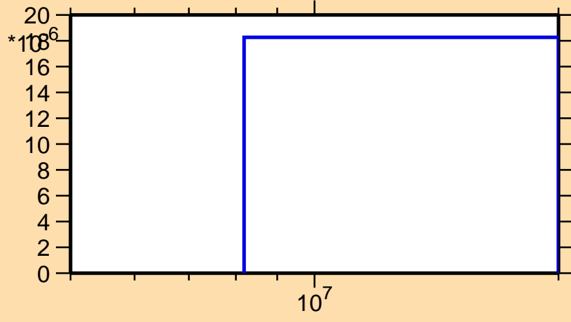
\sigma vs. E for ^{208}\text{Hg}(n,p)
