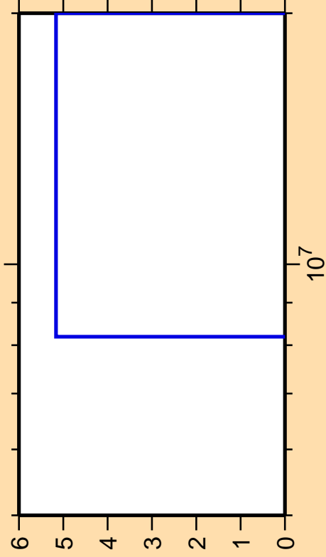
\Delta\sigma/\sigma vs. E for ^{208}\text{Hg}(n,2np)
