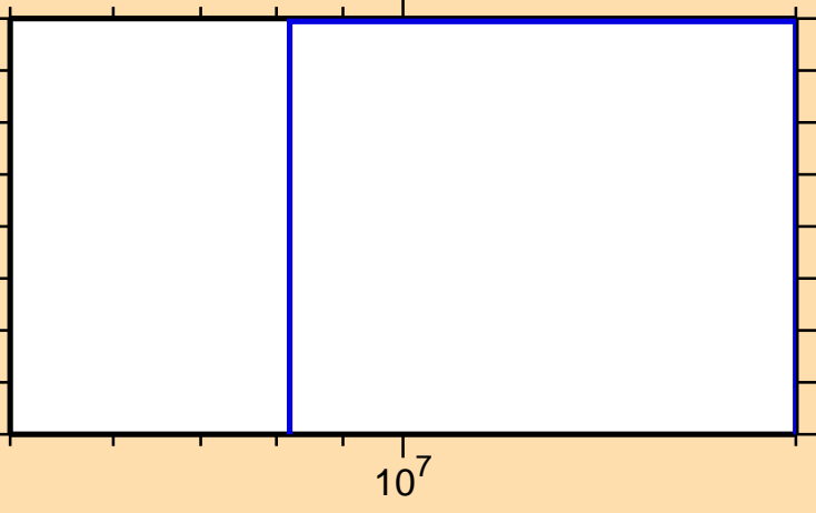
\sigma vs. E for ^{208}\text{Hg}(n,t)
