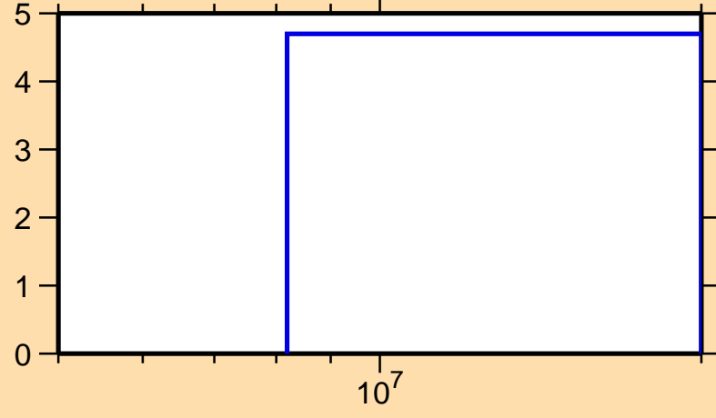
\Delta\sigma/\sigma vs. E for ^{208}\text{Hg}(n,el.)
