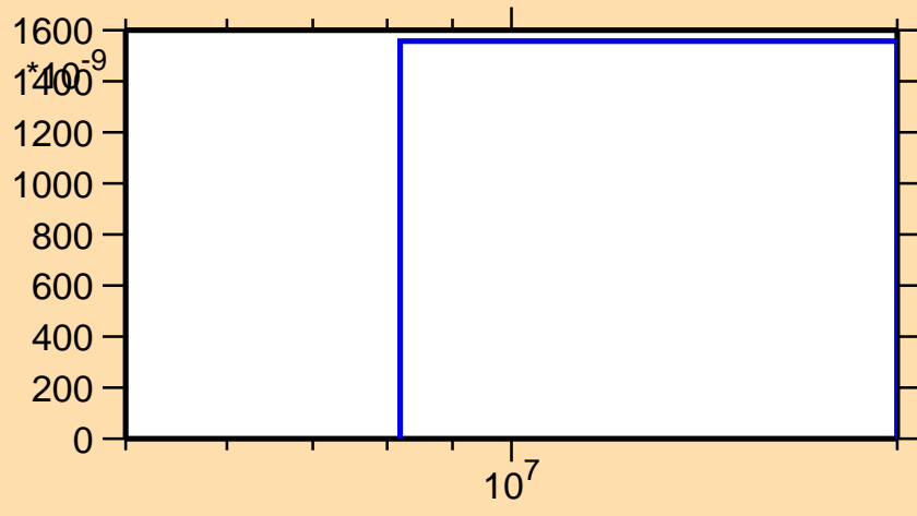
\sigma vs. E for ^{208}\text{Hg}(n,d)
