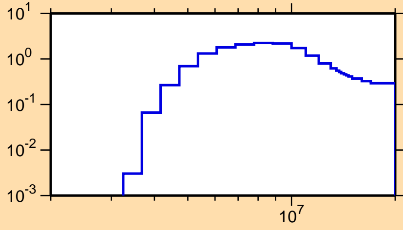
\sigma vs. E for ^{209}\text{Hg}(n,2n)
