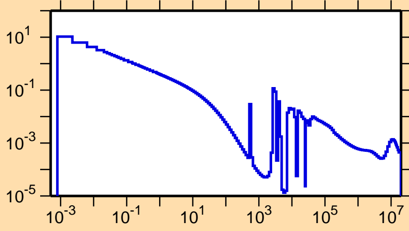
\sigma vs. E for ^{209}\text{Hg}(n,\gamma)
