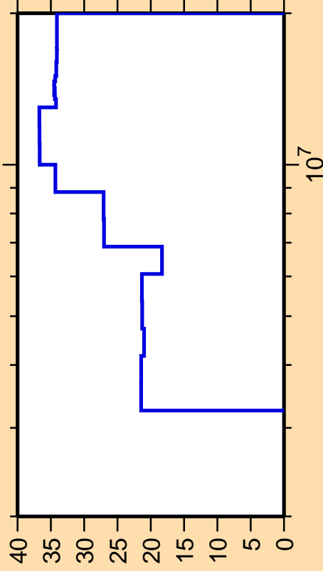
\Delta\sigma/\sigma vs. E for ^{209}\text{Hg}(n,n\text{cont.})
