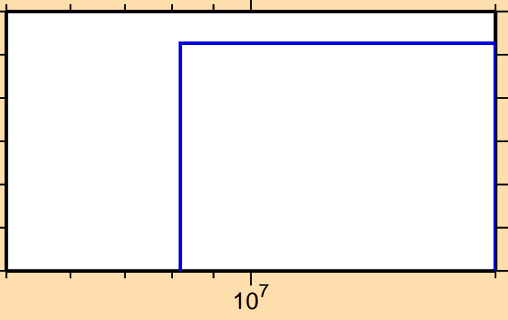
\sigma vs. E for ^{209}\text{Hg}(n,\text{nd})
