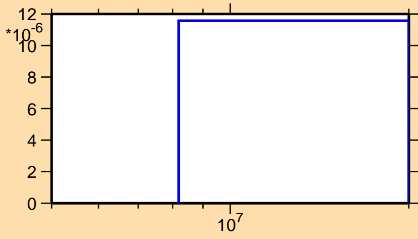
\sigma vs. E for ^{209}\text{Hg}(n,t)
