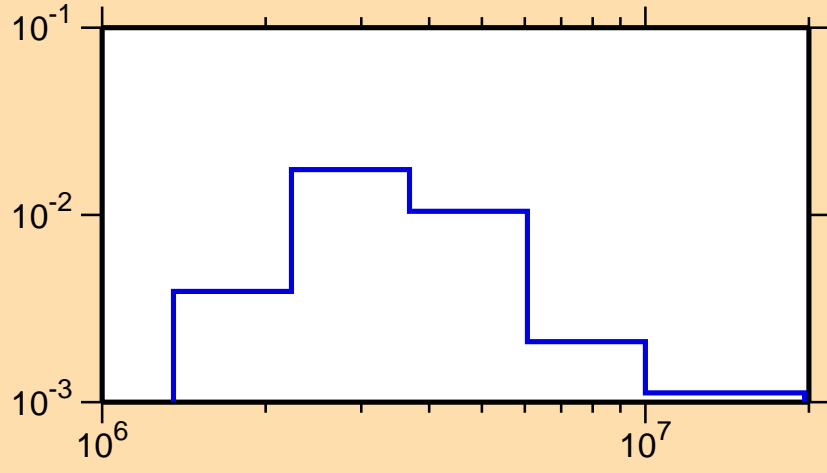
\sigma vs. E for ^{210}\text{Hg}(n,n_4)
