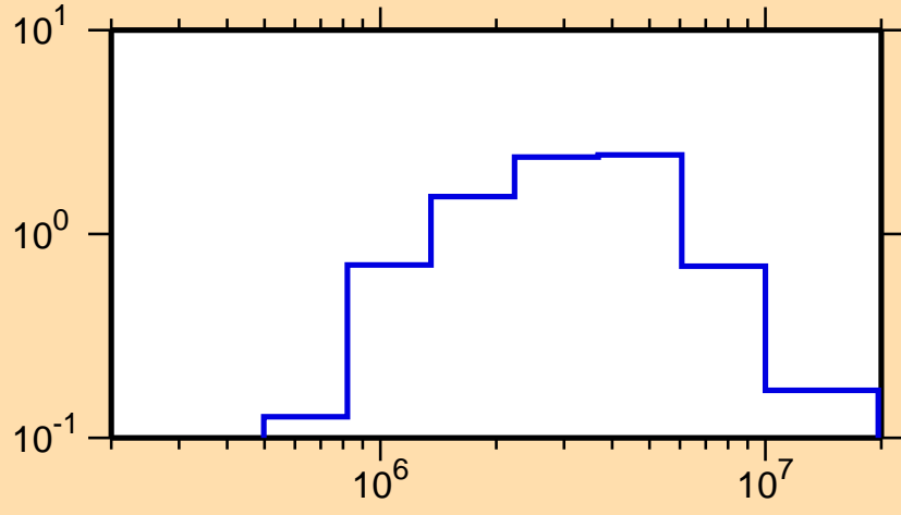
\sigma vs. E for ^{210}\text{Hg}(n,\text{inel.})
