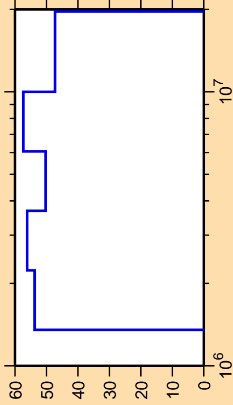
\Delta\sigma/\sigma vs. E for ^{210}\text{Hg}(n,n_4)
