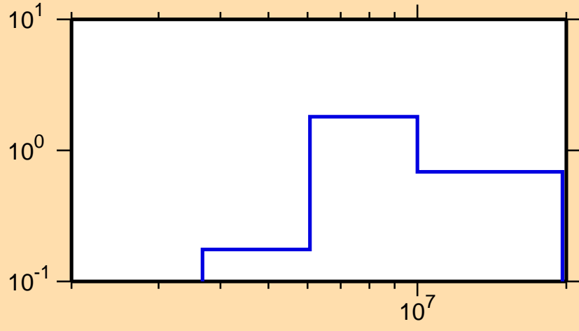
\sigma vs. E for ^{210}\text{Hg}(n,2n)
