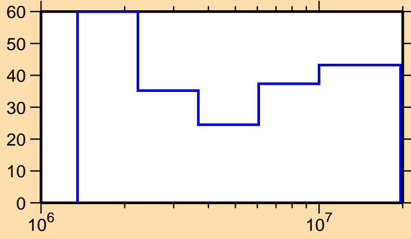
\Delta\sigma/\sigma vs. E for ^{210}\text{Hg}(n,n\text{cont.})
