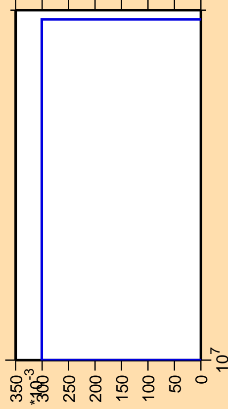
\Delta\sigma/\sigma vs. E for ^{210}\text{Hg}(n,3n\alpha)
