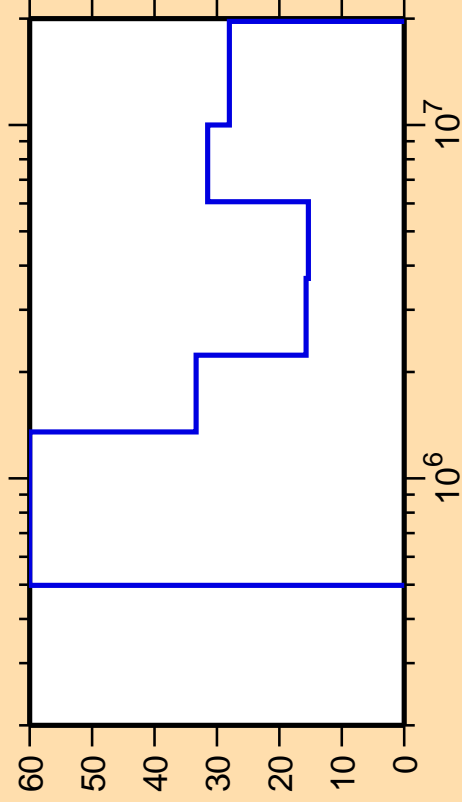
\Delta\sigma/\sigma vs. E for ^{210}\text{Hg}(n,\text{inel.})
