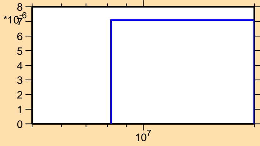
\sigma vs. E for ^{210}\text{Hg}(n,p)
