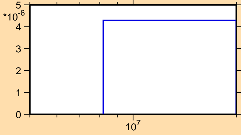
\sigma vs. E for ^{210}\text{Hg}(n,t)
