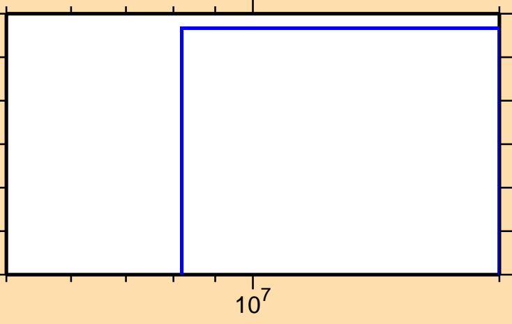
\sigma vs. E for ^{210}\text{Hg}(n,nt)
