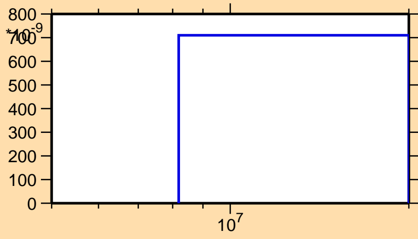
\sigma vs. E for ^{210}\text{Hg}(n,d)
