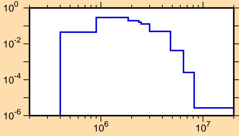
\sigma vs. E for ^{210}\text{Hg}(n,n_2)
