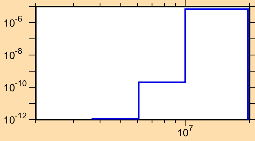
\sigma vs. E for ^{211}\text{Hg}(n,\alpha)
