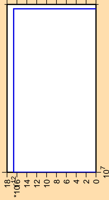
\Delta\sigma/\sigma vs. E for ^{211}\text{Hg} (mt 42)
