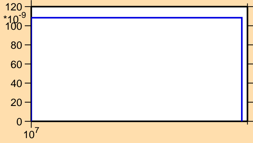
\sigma vs. E for ^{211}\text{Hg}(n,nt)
