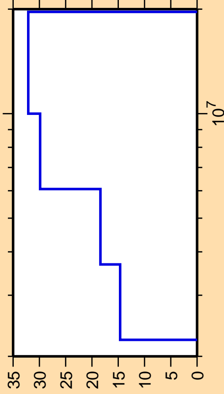
\Delta\sigma/\sigma vs. E for ^{211}\text{Hg}(n,n\text{cont.})
