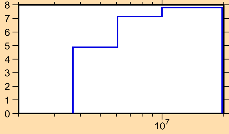
\Delta\sigma/\sigma vs. E for ^{211}\text{Hg}(n,\text{nonel.})
