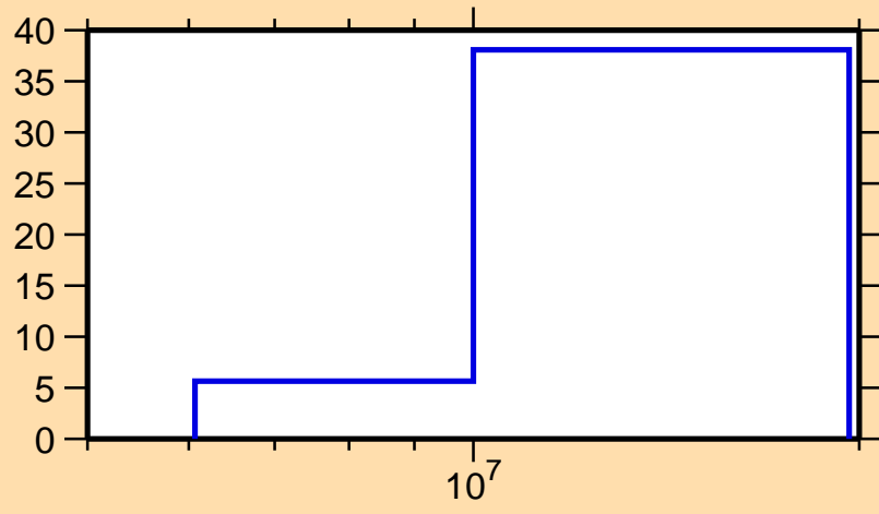
\Delta\sigma/\sigma vs. E for ^{211}\text{Hg}(n,2n)
