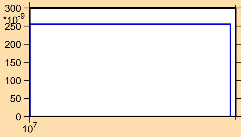
\sigma vs. E for ^{211}\text{Hg}(n,np)
