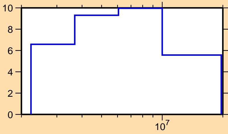
\Delta\sigma/\sigma vs. E for ^{211}\text{Hg}(n,\text{tot.})
