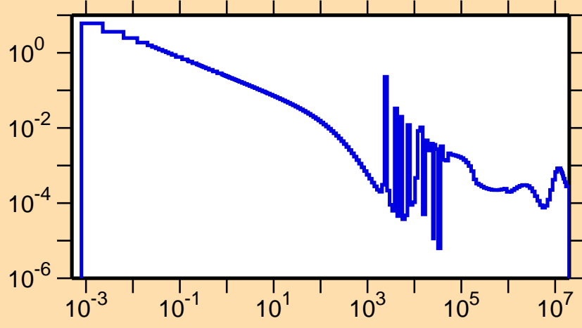
\sigma vs. E for ^{212}\text{Hg}(n,\gamma)
