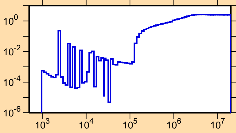
\sigma vs. E for ^{212}\text{Hg}(n,\text{nonel.})
