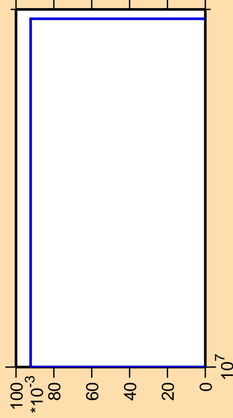
\Delta\sigma/\sigma vs. E for ^{212}\text{Hg}(n,2np)
