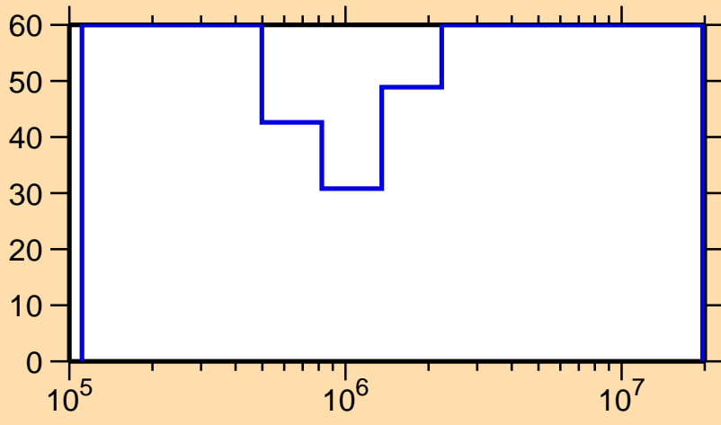
\Delta\sigma/\sigma vs. E for ^{212}\text{Hg}(n,n_1)
