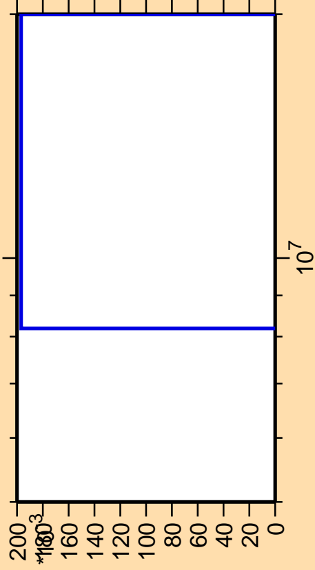
\Delta\sigma/\sigma vs. E for ^{212}\text{Hg}(n,3n\alpha)
