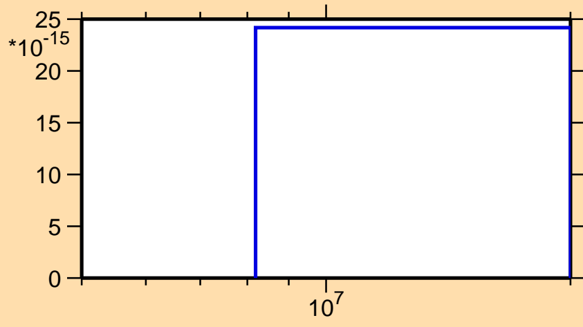
\sigma vs. E for ^{212}\text{Hg}(n,3n\alpha)
