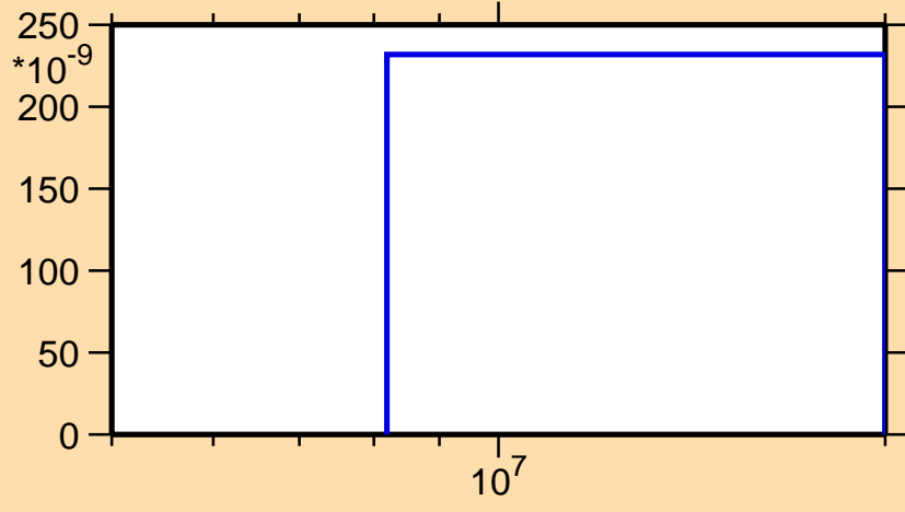
\sigma vs. E for ^{212}\text{Hg}(n,n\alpha)
