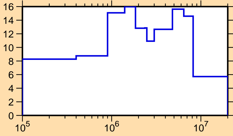
\Delta\sigma/\sigma vs. E for ^{212}\text{Hg}(n, el.)
