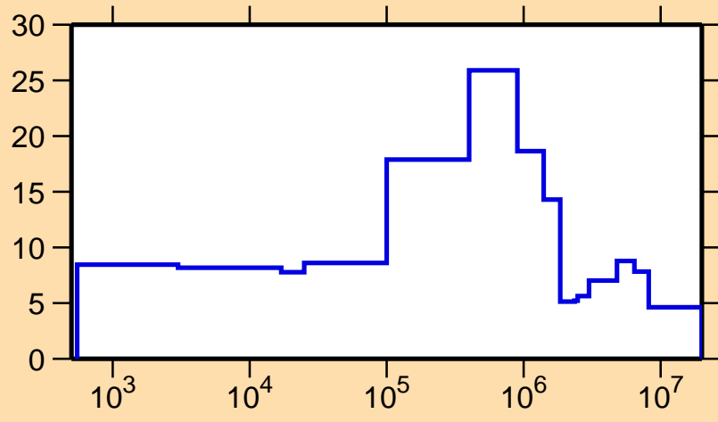
\Delta\sigma/\sigma vs. E for ^{212}\text{Hg}(n,\text{tot.})
