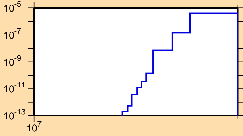
\sigma vs. E for ^{213}\text{Hg}(n,nt)
