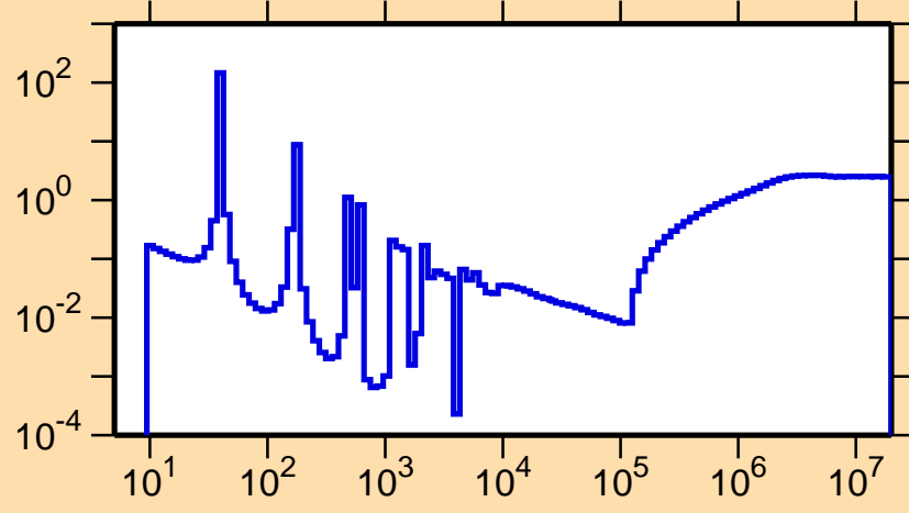
\sigma vs. E for ^{213}\text{Hg}(n,\text{nonel.})
