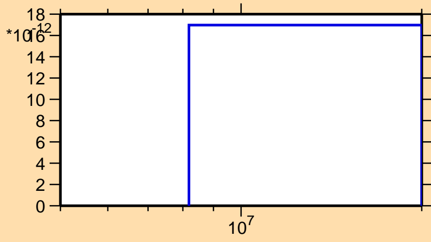
\sigma vs. E for ^{213}\text{Hg}(n,2np)
