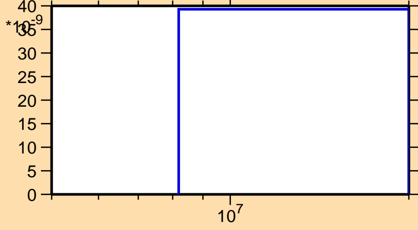
\sigma vs. E for ^{213}\text{Hg}(n,nt)
