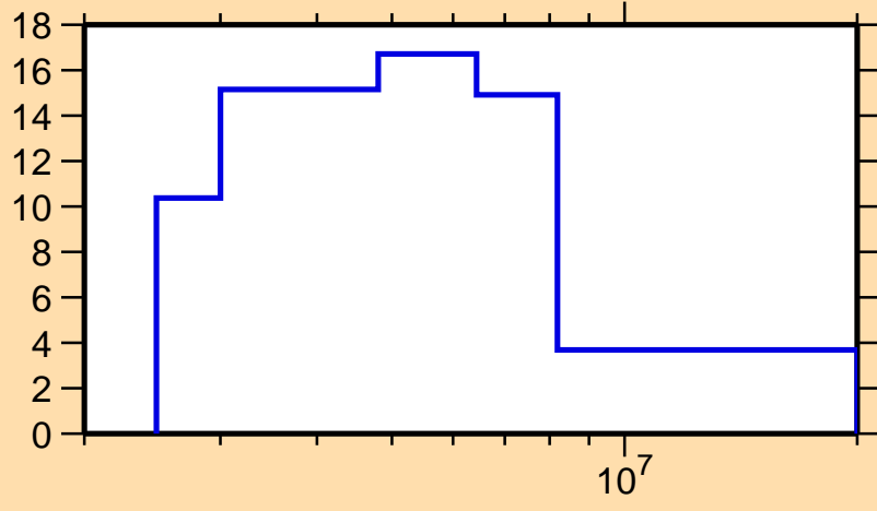
\Delta\sigma/\sigma vs. E for ^{213}\text{Hg}(n,\text{tot.})
