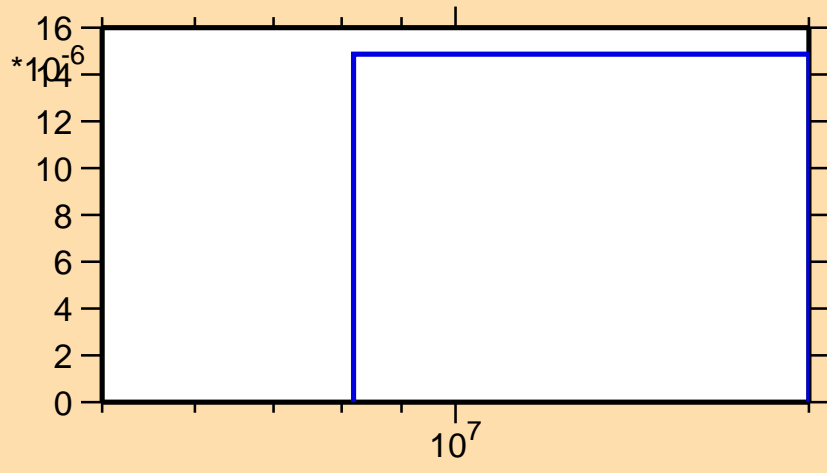
\sigma vs. E for ^{213}\text{Hg}(n,p)
