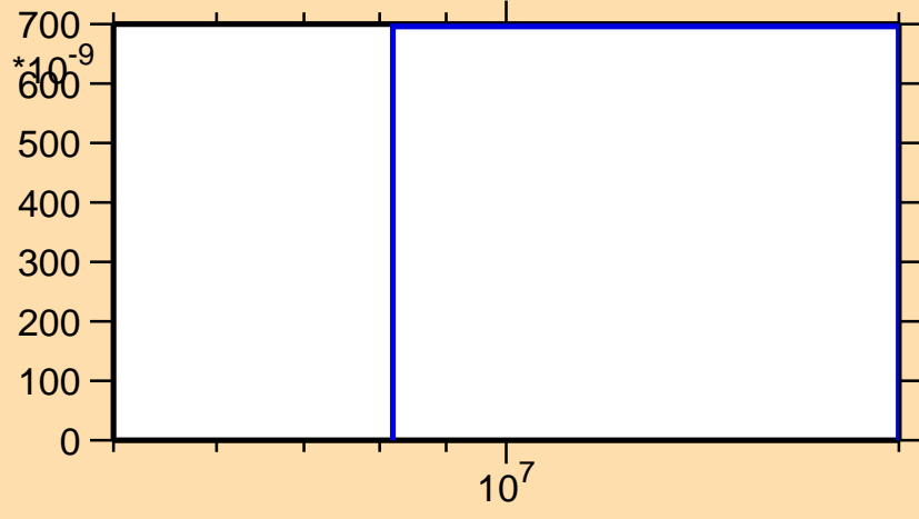
\sigma vs. E for ^{213}\text{Hg}(n,n\alpha)
