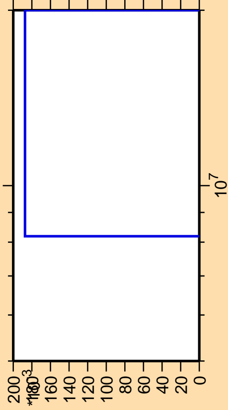
\Delta\sigma/\sigma vs. E for ^{213}\text{Hg}(n,3n\alpha)
