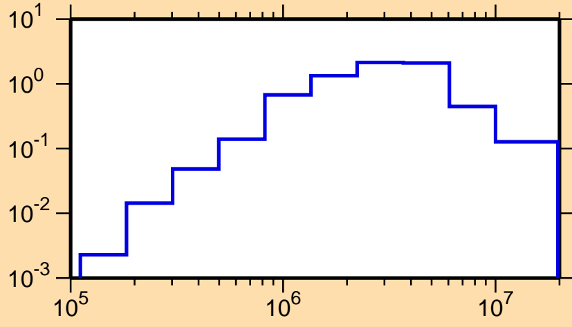
\sigma vs. E for ^{214}\text{Hg}(n,n\text{cont.})
