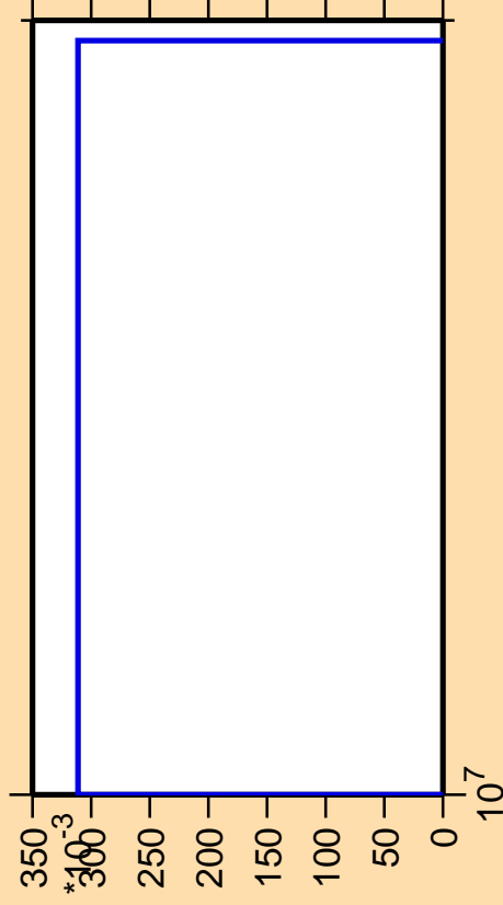
\Delta\sigma/\sigma vs. E for ^{214}\text{Hg}(n,2np)
