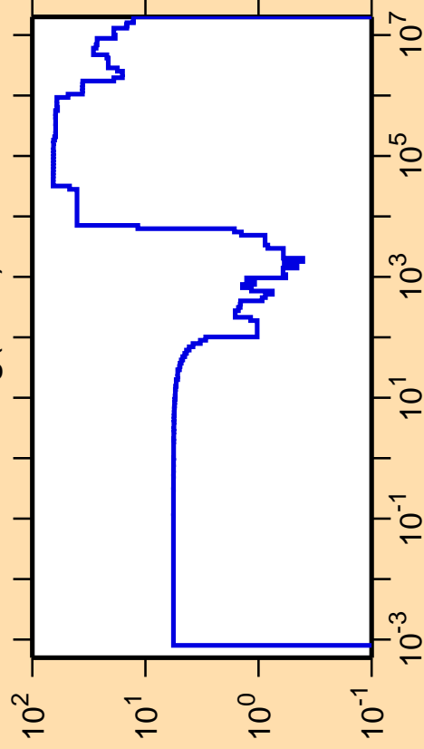
\Delta\sigma/\sigma vs. E for ^{215}\text{Hg}(n,\text{el.})
