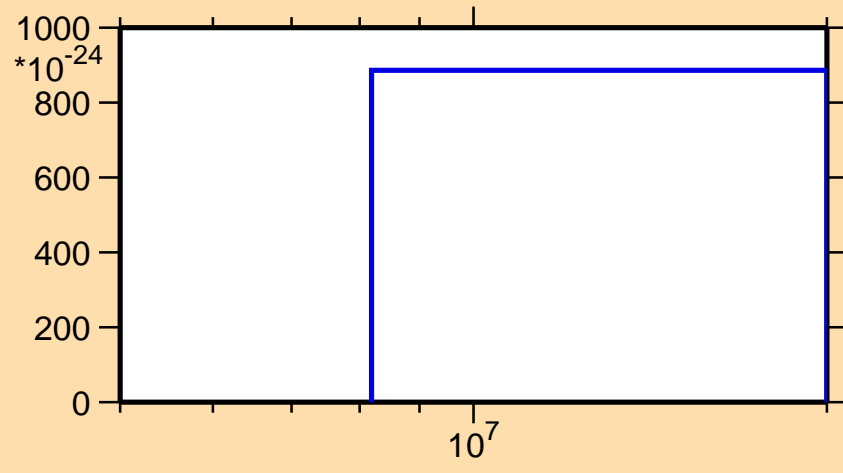
\sigma vs. E for ^{215}\text{Hg} (mt 42)
