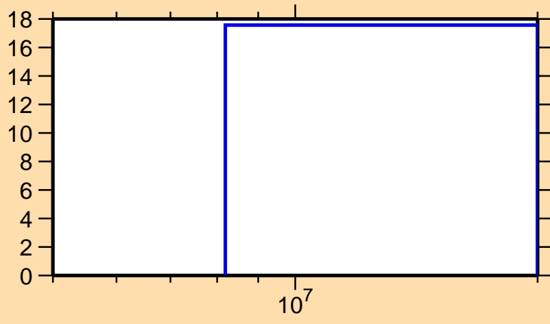
\Delta\sigma/\sigma vs. E for ^{215}\text{Hg}(n,2n)
