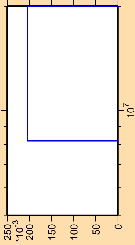
\Delta\sigma/\sigma vs. E for ^{215}\text{Hg}(n,3n\alpha)
