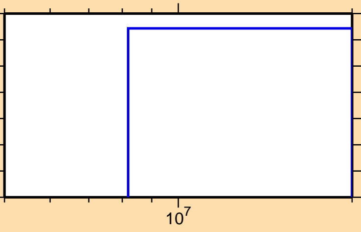
\sigma vs. E for ^{215}\text{Hg}(n,\text{nd})
