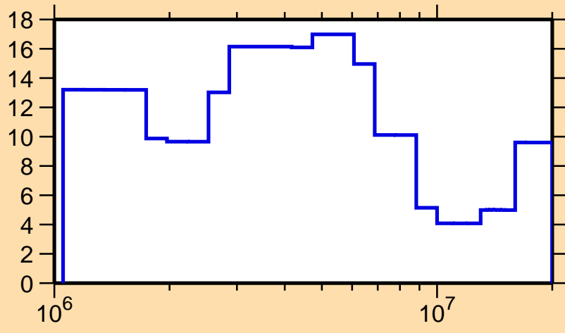
\Delta\sigma/\sigma vs. E for ^{145}\text{Ho}(n,\text{tot.})
