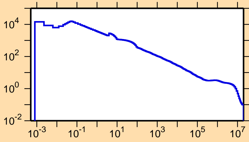
\sigma vs. E for ^{145}\text{Ho}(n,p)
