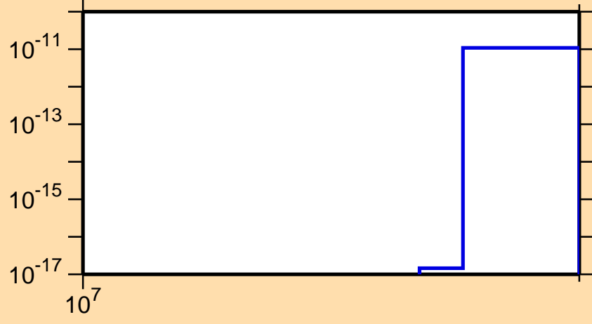
\sigma vs. E for ^{145}\text{Ho}(n,nt)
