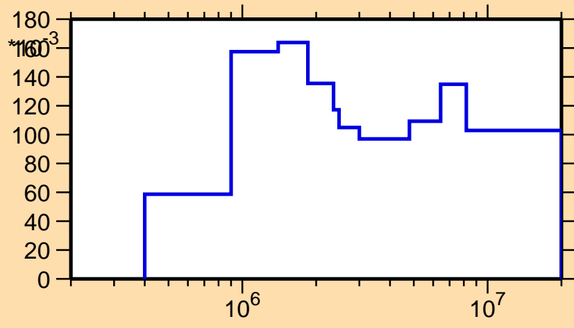
\sigma vs. E for ^{145}\text{Ho}(n,\text{inel.})
