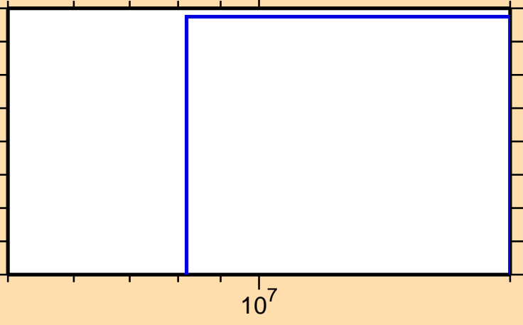
\sigma vs. E for ^{145}\text{Ho}(n,\text{nd})
