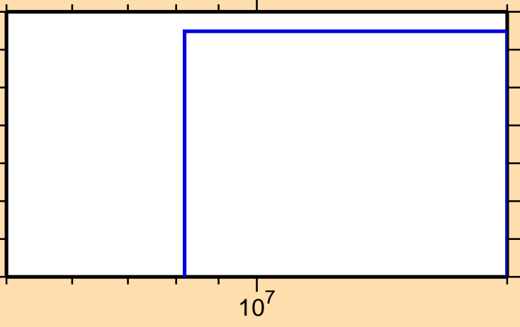
\sigma vs. E for ^{145}\text{Ho}(n,2n)
