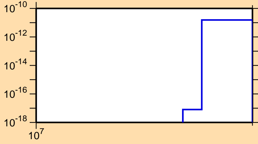
\sigma vs. E for ^{146}\text{Ho}(n,nt)
