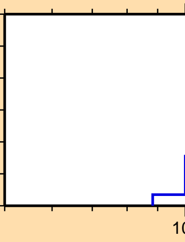
\sigma vs. E for ^{146}\text{Ho}(\text{mt117})
