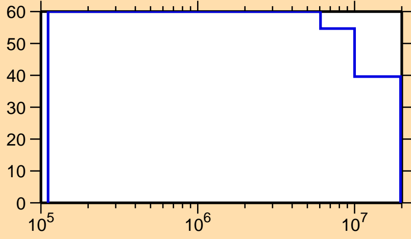
\Delta\sigma/\sigma vs. E for ^{146}\text{Ho}(n,n\text{cont.})
