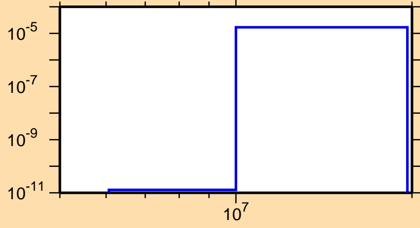
\sigma vs. E for ^{146}\text{Ho} (mt 45)
