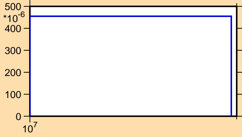
\sigma vs. E for ^{146}\text{Ho}(n,2np)
