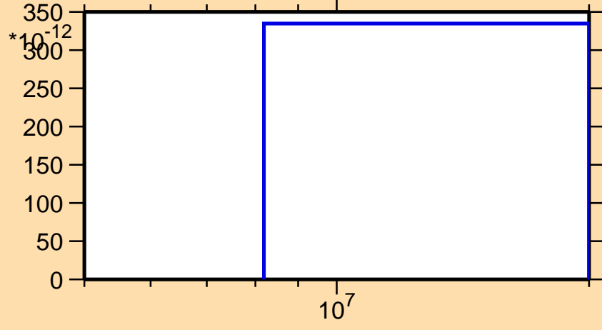
\sigma vs. E for ^{146}\text{Ho}(\text{mt } 34)
