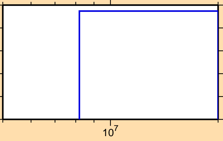
\sigma vs. E for ^{146}\text{Ho}(n,2n)
