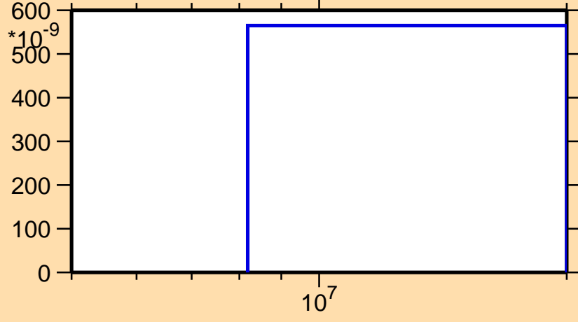
\sigma vs. E for ^{146}\text{Ho}(n,\text{pt})
