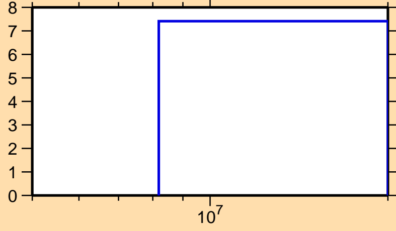
\Delta\sigma/\sigma vs. E for ^{146}\text{Ho}(n,\text{el.})
