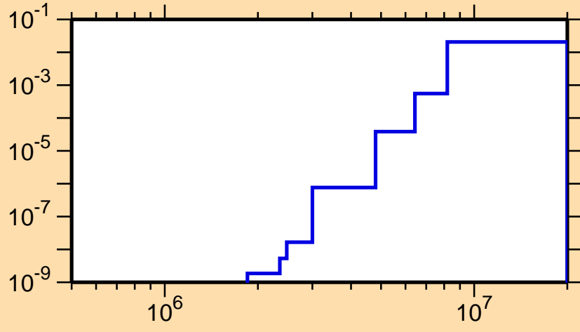
\sigma vs. E for ^{146}\text{Ho}(n,d)
