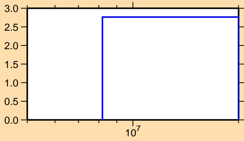
\Delta\sigma/\sigma vs. E for ^{146}\text{Ho}(n,\text{tot.})
