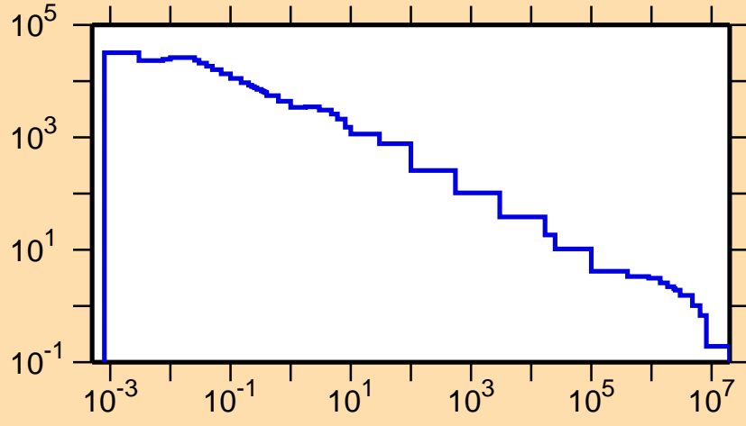
\sigma vs. E for ^{146}\text{Ho}(n,p)
