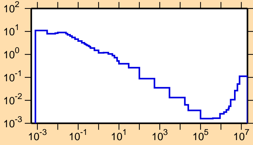
\sigma vs. E for ^{146}\text{Ho}(n,\alpha)
