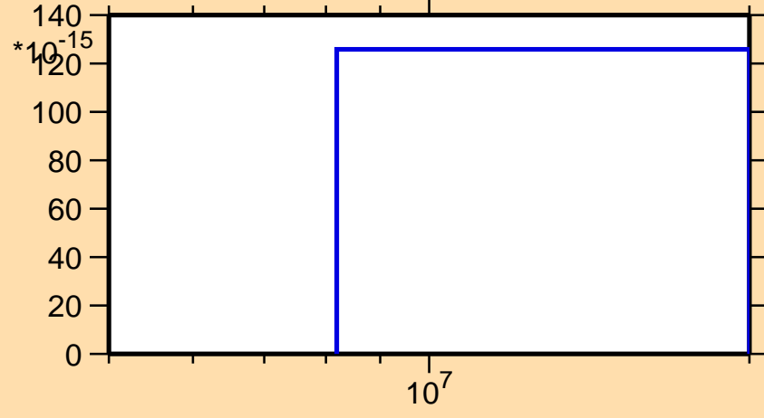
\sigma vs. E for ^{146}\text{Ho}(n,nt)
