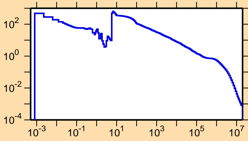
\sigma vs. E for ^{147}\text{Ho}(n,\gamma)
