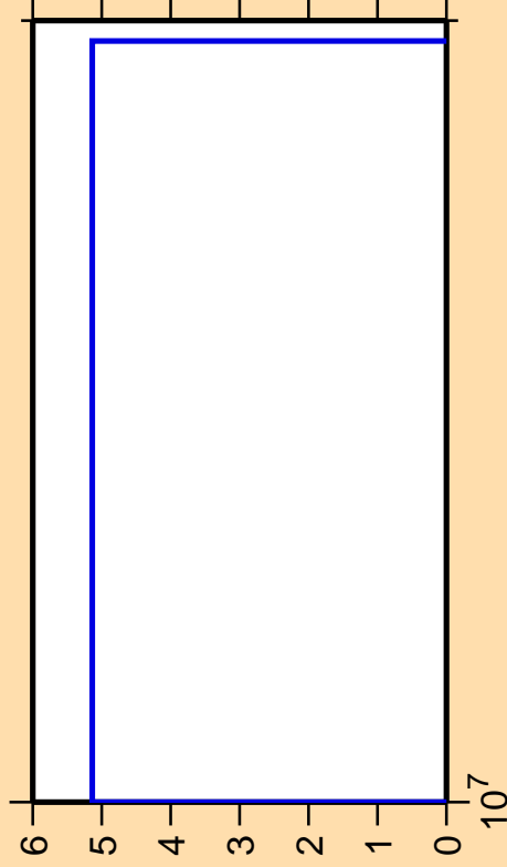
\Delta\sigma/\sigma vs. E for ^{147}\text{Ho} (mt 34)
