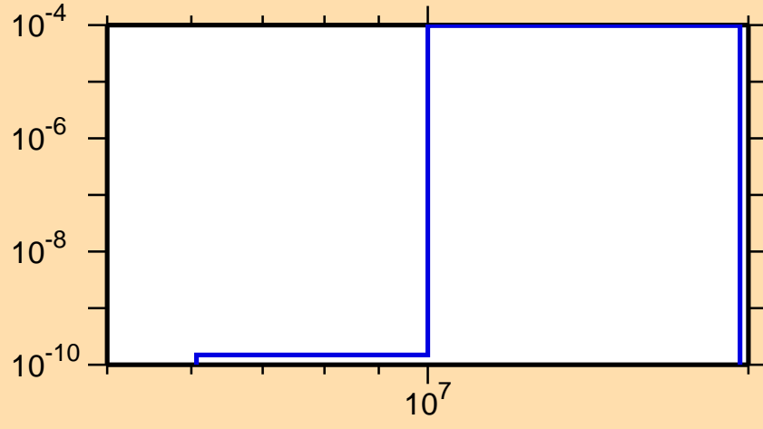
\sigma vs. E for ^{147}\text{Ho}(n,\text{pd})
