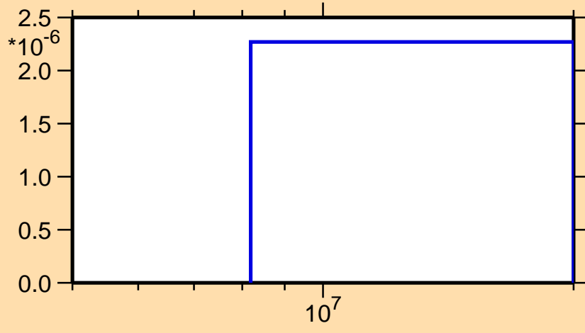
\sigma vs. E for ^{147}\text{Ho} (mt 45)
