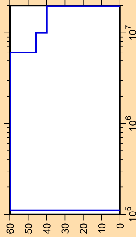
\Delta\sigma/\sigma vs. E for ^{148}\text{Ho}(n,\text{inel.})
