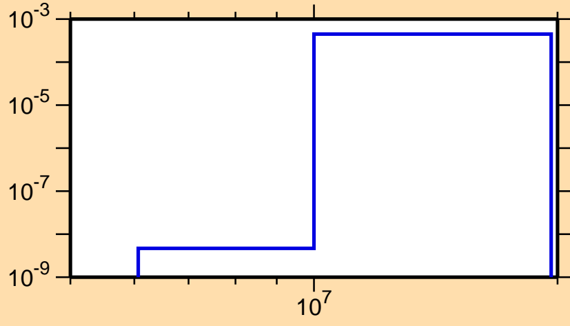
\sigma vs. E for ^{148}\text{Ho}(n,t)
