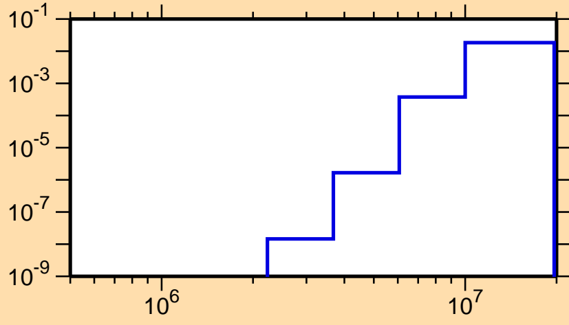
\sigma vs. E for ^{148}\text{Ho}(n,d)
