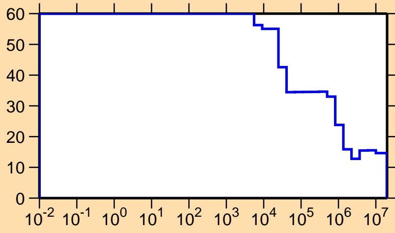
\Delta\sigma/\sigma vs. E for ^{148}\text{Ho}(n,\text{nonel.})
