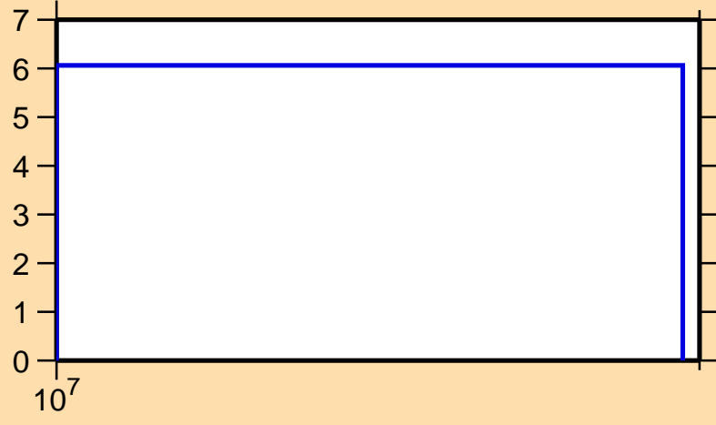
\Delta\sigma/\sigma vs. E for ^{148}\text{Ho}(n,\text{tot.})
