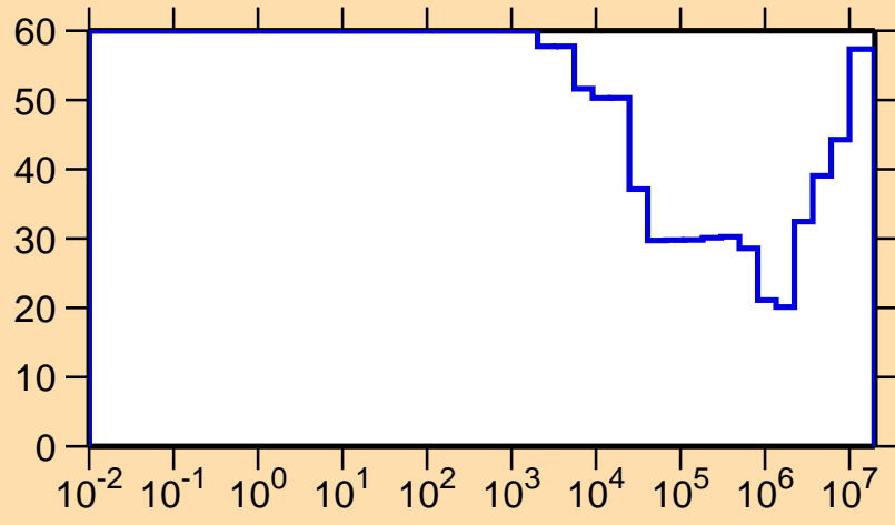
\Delta\sigma/\sigma vs. E for ^{148}\text{Ho}(n,p)
