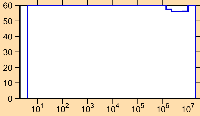
\Delta\sigma/\sigma vs. E for ^{148}\text{Ho}(n,n_1)
