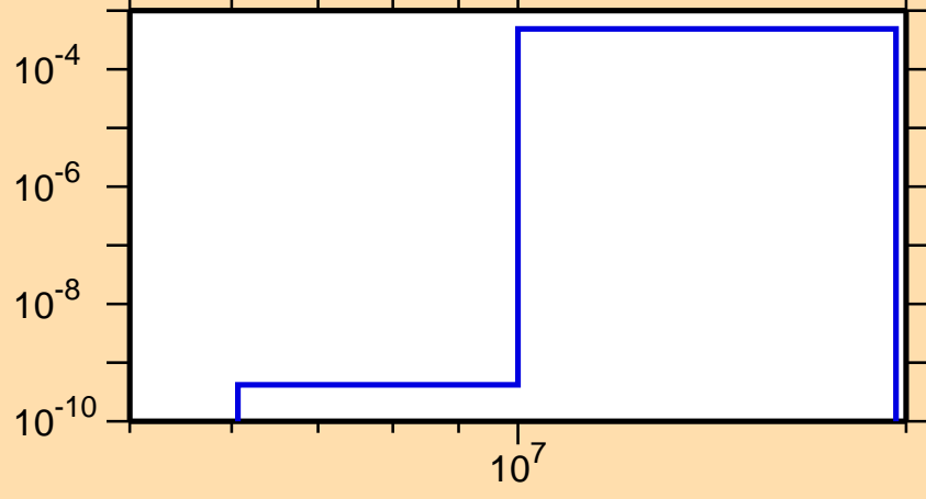
\sigma vs. E for ^{148}\text{Ho}(n,t)
