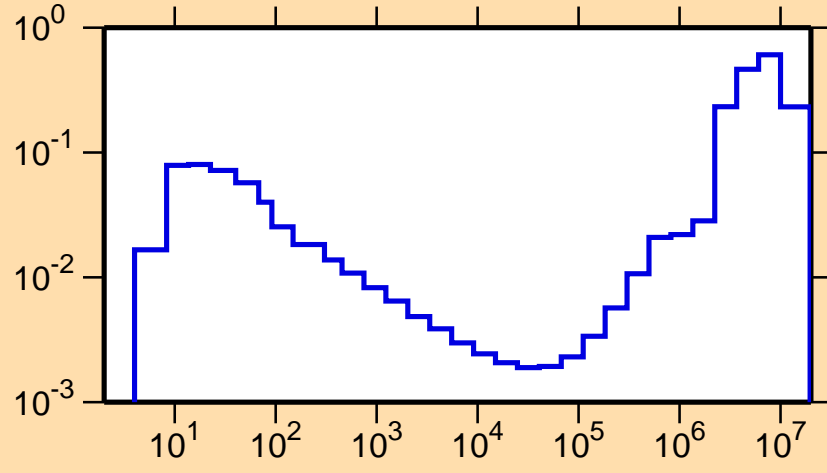
\sigma vs. E for ^{148}\text{Ho}(n,\text{inel.})
