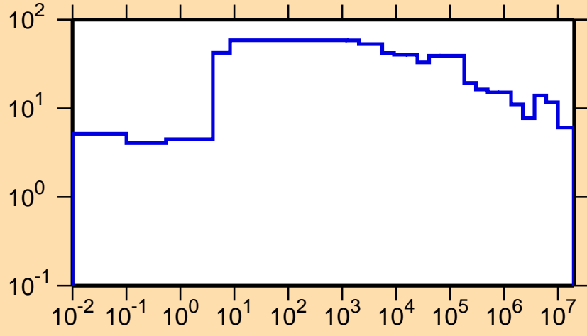
\Delta\sigma/\sigma vs. E for ^{148}\text{Ho}(n,\text{tot.})
