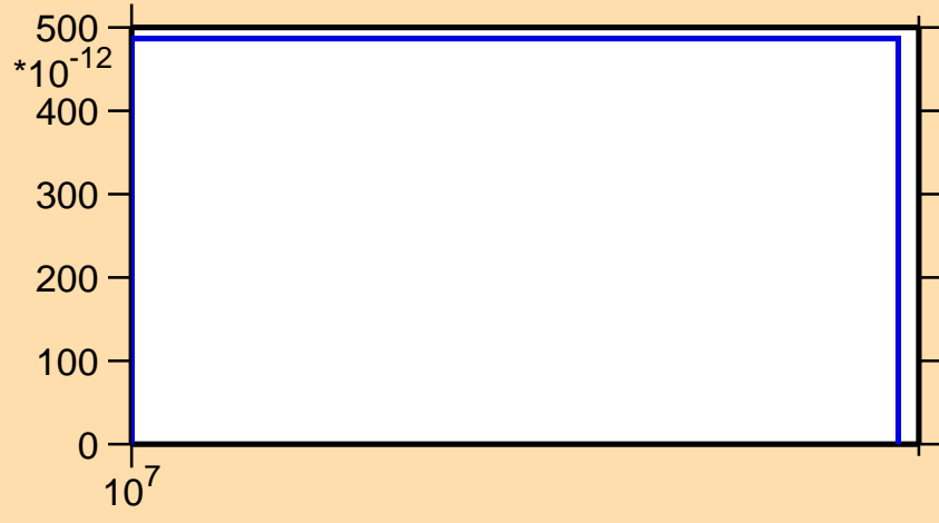
\sigma vs. E for ^{148}\text{Ho}(n,2n\alpha)
