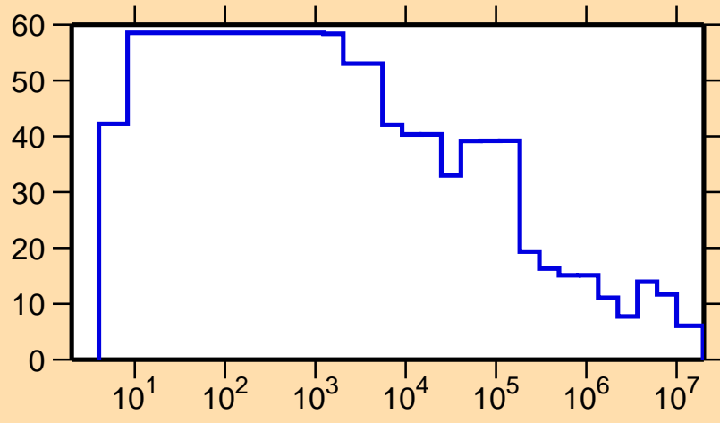
\Delta\sigma/\sigma vs. E for ^{148}\text{Ho}(n,\text{tot.})
