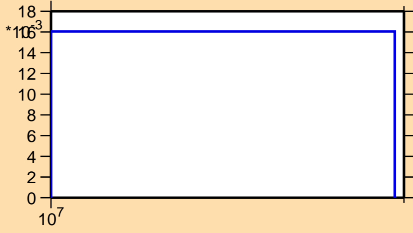
\sigma vs. E for ^{148}\text{Ho}(n,2n)
