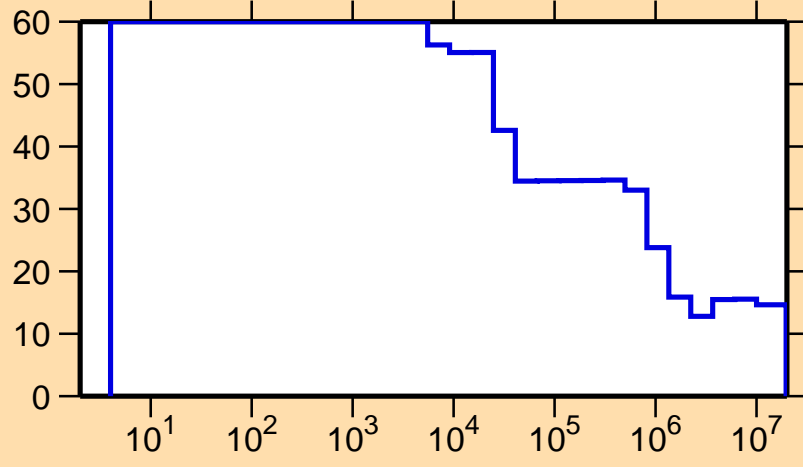
\Delta\sigma/\sigma vs. E for ^{148}\text{Ho}(n,\text{nonel.})
