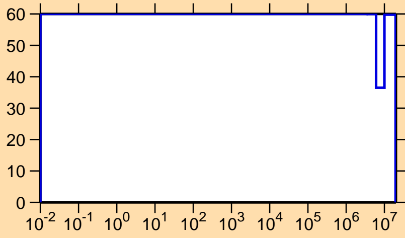
\Delta\sigma/\sigma vs. E for ^{148}\text{Ho}(n,n\text{cont.})
