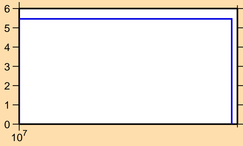
\Delta\sigma/\sigma vs. E for ^{148}\text{Ho}(n,\text{el.})
