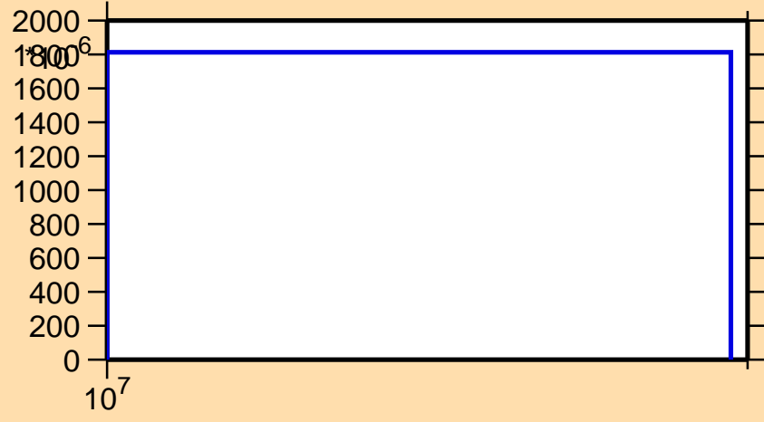
\sigma vs. E for ^{148}\text{Ho}(n,2np)
