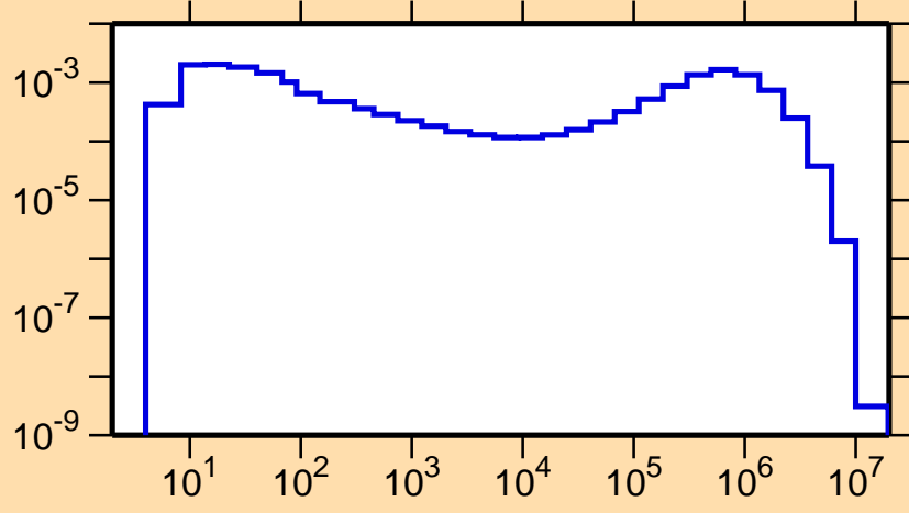
\sigma vs. E for ^{148}\text{Ho}(n,n_2)
