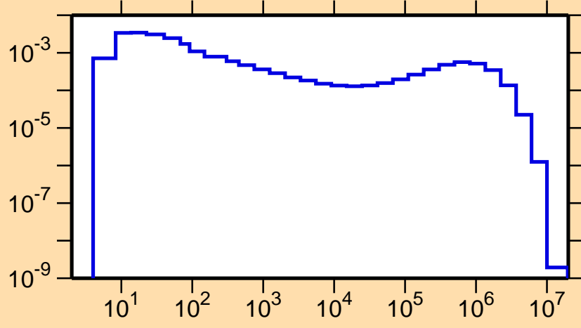
\sigma vs. E for ^{148}\text{Ho}(n,n_1)
