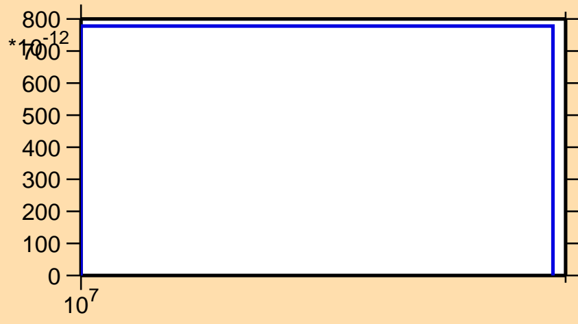
\sigma vs. E for ^{148}\text{Ho} (mt 34)
